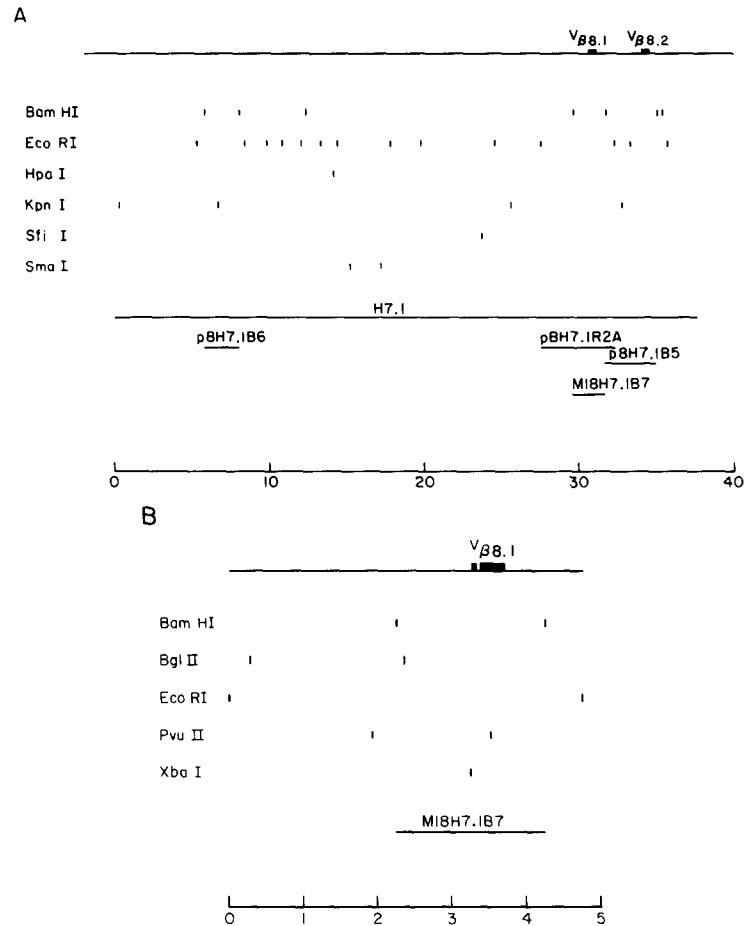
FIGURE 2. Restriction maps of the cosmid and \lambda clones containing the members of the V_{\beta 8} family. (A) Cosmid H7.1, containing V_{\beta 8.1} and V_{\beta 8.2} , and the pBR322 subclone pBH7.1R2A, the pUC8 subclones p8H7.1B6 and p8H7.1B5, and the M13mp18 subclone M18H7.1B7 of this region. (B) Plasmid pBH7.1R2A, containing the V_{\beta 8.1} gene segment, and the M13mp18 subclone M18H7.1B7. (C) Cosmids H18.1 and H9.1, containing V_{\beta 8.4} , and the pBR322 subclone pBH9.1R3 and the pUC8 subclone p8H18.1RH that contains portions of these cosmids. (D) \lambda VB8.5, containing the V_{\beta 8.5} gene segment, and the M13mp18 subclone M18VB8.5 that contains a portion of this region. (E) \lambda gt7 clone \lambda VB8.3, containing the V_{\beta 8.3} gene segment. Scale in each figure is in kb. The thin and thick boxes represent the first and second exons of the germline V_{\beta} gene segment.
