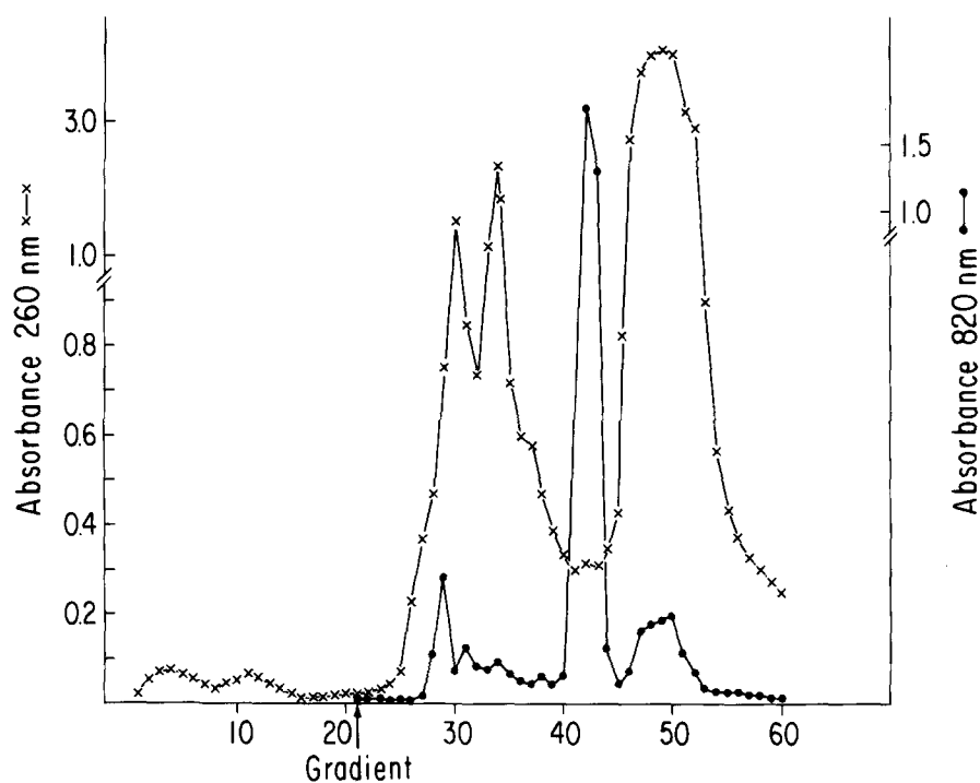
FIG. 3. Separation of the components of the Tris-released material from N. gonorrhoeae R10 on a DEAE-Sephacose column. Chromatography was performed in 10 mM Tris-HCl pH 8.0, 1 mM EDTA, with a linear gradient of NaCl from 0 to 1.0 M. The eluate was monitored for absorbance at 260 nm, and for phosphorus content.
