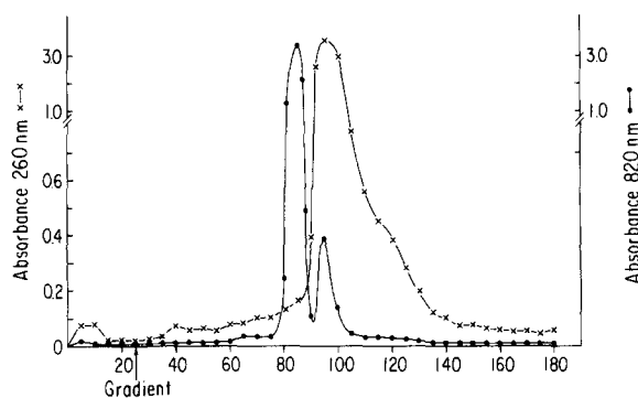
FIG. 1. Separation of the components of NaOCl-extracted N. gonorrhoeae R10 on a DEAE-Sepharose column. Chromatography was performed in 10 mM Tris-HCl pH 8.0, 1 mM EDTA, with a linear NaCl gradient from 0 to 1 M. The fractions were monitored for absorbance at 260 nm, and for phosphorus content.
