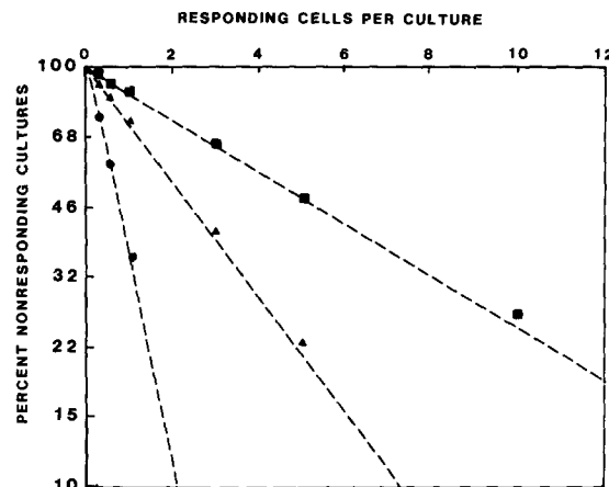
FIG. 5. Frequency analysis of the precursors of proliferating T cells with cytolytic potential. After 18 d of culture, each microculture was scored microscopically for growth (●) and then was split into two aliquots which were tested against either murine P815 target cells in the presence of PHA (▲) or human K562 target cells (■). Each point is based on a group of 54 microcultures. The regression lines were fitted to the data by the minimum \chi^2 method.
