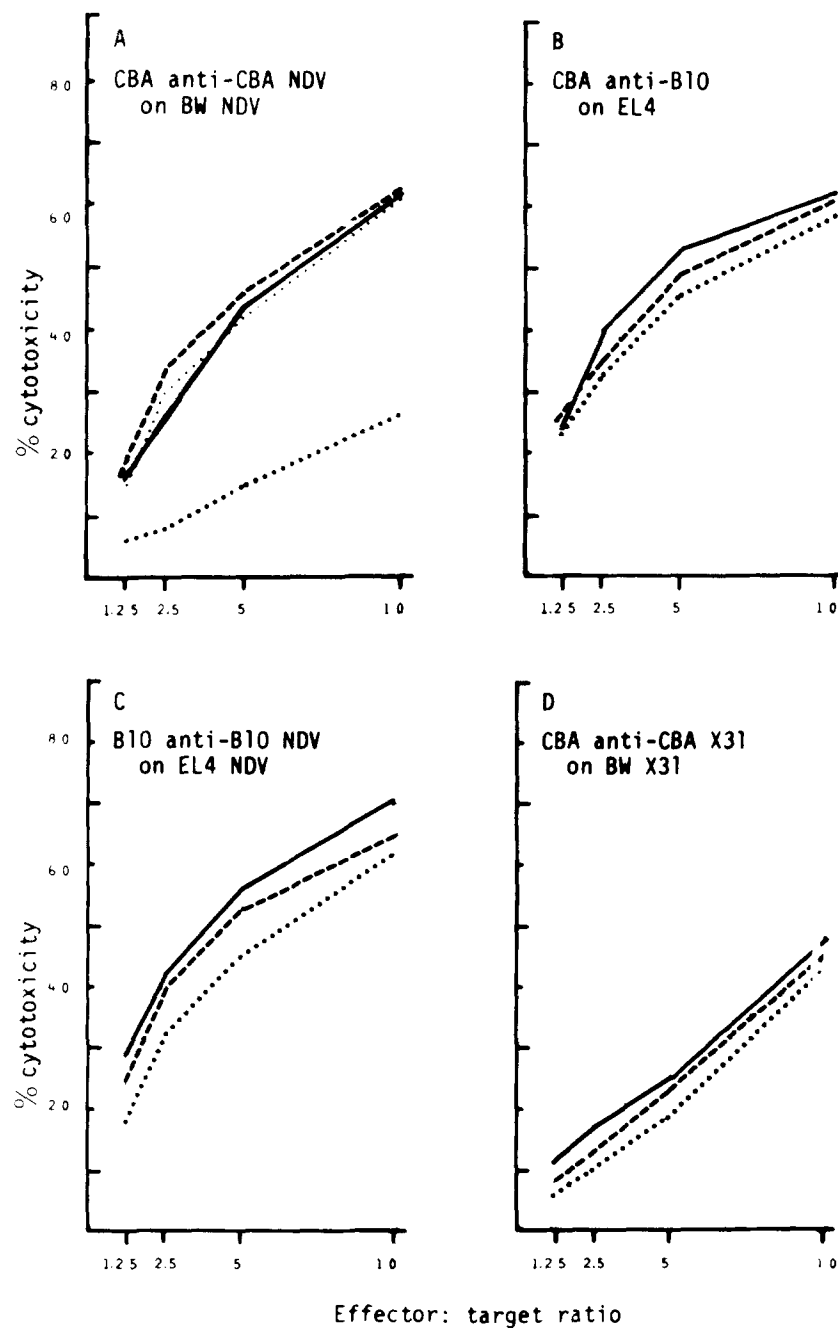
FIG. 3. Cytotoxicity of four different CTL populations tested on appropriate target cells after treatment with anti-id serum CBA-113 and complement (···), NMS and complement (---), serum CBA-113 alone (-.-), or left untreated (—).
