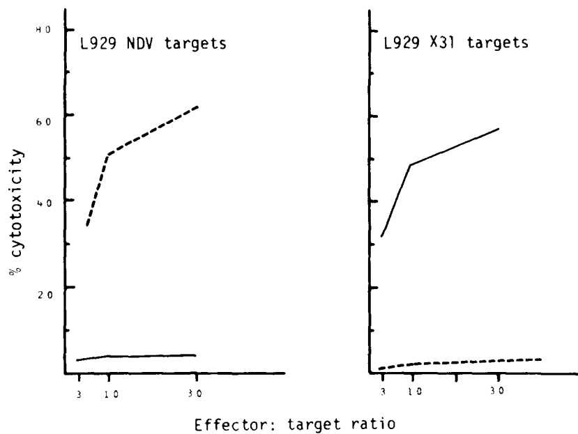
FIG. 2. Virus specificity of NDV- and X31-immune CTL. CBA anti-CBA NDV CTL (---) and CBA anti-CBA X31 CTL (—) were assayed on NDV-infected L929 target cells (left panel) and on X31-infected L929 target cells (right panel).
