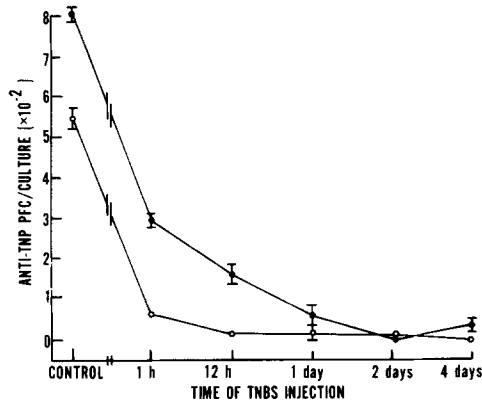
FIG. 4. Kinetics of TNBS tolerance: challenge with TNP-Ficoll in vitro . Information is identical to Fig. 1 except that TNP-Ficoll was utilized rather than TNP-LPS. The anti-TNP PFC per culture responses were: TNBS day 4: 777 ± 26; TNBS day 2: 810 ± 33; TNBS day 1: 880 ± 53; TNBS 12 h: 986 ± 27; TNBS 1 h: 829 ± 36; and no TNBS: 760 ± 29. Data from two experiments are pooled. O, TNP-LPS; ●, TNP-Ficoll.
