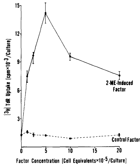
FIG. 3. Dose dependency of the DNA synthetic response to 2-ME-induced soluble factor. 5 \times 10^5 viable C3H/St spleen cells were cultured for 2 d in 0.1 ml of control- or 2-ME-induced soluble factor containing an incremental number of cell-equivalents/ml. Cells were pulsed with 1.0 \mu\text{Ci} of [ ^3\text{H} ]TdR (6.7 Ci/mM) for the final 24 h of culture. Results are expressed as the arithmetic mean of five replicate cultures \pm the standard error.
