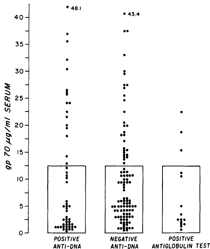
Fig. 3. Serum gp70 levels of the NZB \times SWR crosses in relation to presence or absence of anti-DNA antibody (positive = >10% binding to either nDNA and/or dDNA) and positive antiglobulin (direct Coombs'). The value of 10% binding is 2 SD above the mean for SWR mice. Open box separates values for serum gp70 above and below 12.5 \mu\text{g/ml} . Each closed circle is one animal.
