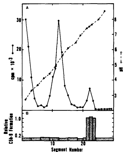
FIG. 5. Localization of complement-activating ability to a protein with pI 7.5. Surface-labeled, sucrose density-banded, virus was disrupted in 1% Triton X-100 and centrifuged at 160,000 g_{max} for 10 min. The supernate was then subjected to IEF in Pevikon/Sephadex G-75 containing 0.2% Triton X-100 and 2% ampholines ( pH 4–9). After division of the bed into 30 equal segments, pH and radioactivity of each segment were determined (A). The carrier material was removed by filtration, and each fraction was neutralized and freed of ampholines by dialysis against PBS containing 0.1% Triton X-100. The ability of each fraction to form C5b-9 was then determined (B).
