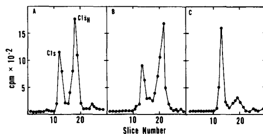
FIG. 6. Conversion of C1 to C1_i by the viral activator. The fraction at pH 7.5 of Fig. 5 was isolated, dialyzed and freed of Triton X-100 by passage through SM-2 Bio-Beads (Bio-Rad Laboratories, Richmond, Calif.). One-half of the sample ( 50 \mu l ) was then incubated with 50 \mu l of C1 containing ^{125}I -C1s for 30 min at 37^\circ C in the absence (A) or in the presence (B) of 0.1% Triton X-100. Under these conditions activation of C1 results in proteolytic cleavage of C1s to form C1_i s. The labeled, heavy chain ( C1_{iH} ) of C1_i s can be identified by SDS-PAGE under reducing conditions. (The light chain of C1_i s is not susceptible to radioiodination; for further experimental details see reference 8). The extent of nonspecific C1s conversion by 0.1% Triton X-100 in buffer is shown in C.
