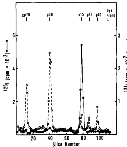
FIG. 7. Characterization of purified viral complement receptor by SDS-PAGE. The dialyzed receptor, purified by IEF from surface-labeled M-MuLV, was labeled with ^{125}\text{I} (●) and then mixed with ^{131}\text{I} -labeled, disrupted M-MuLV (○). Electrophoresis was carried out in 15% polyacrylamide gels in the presence of 0.1% SDS under reducing conditions. Unfixed gels were sliced into 0.7-mm segments. Note the absence of contaminating proteins in the receptor preparation.
