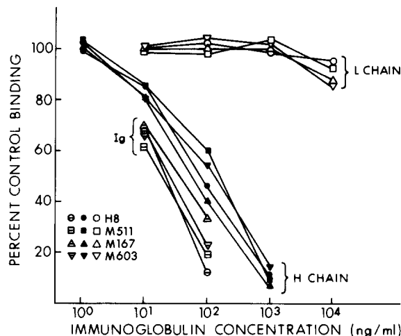
FIG. 3. Location of V_H -PC on the heavy chain. Unfractionated myeloma proteins and heavy and light chains derived from them were tested for inhibition of binding of [ ^{125} I]M167 to Cl anti-H8.
