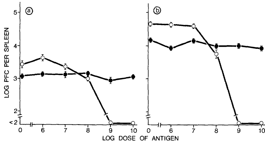
FIG. 2. Numbers of 19S (group a) and 7S (group b) PFC in spleens of irradiated mice 7 days after intravenous injection of 5 \times 10^8 SRC and 5 \times 10^8 HRC given together with 10^7 TDL from mice primed 1 day previously with varying numbers of SRC injected intravenously. \circ = anti-SRC PFC; \bullet = anti-HRC PFC. Geometric means of the results obtained from 4 to 6 mice are given and vertical bars represent upper and lower limits of SE.
