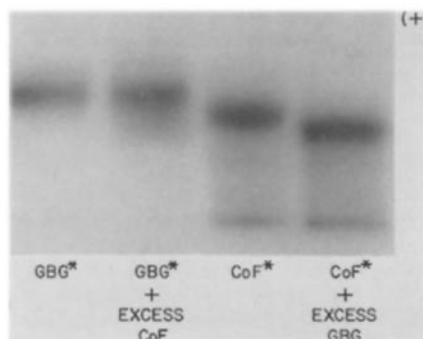
FIG. 6. Autoradiography of polyacrylamide gel electrophoresis of mixtures of purified ^{125}\text{I} -labeled and unlabeled CoF and GBG. Labeled proteins are indicated by asterisks.
