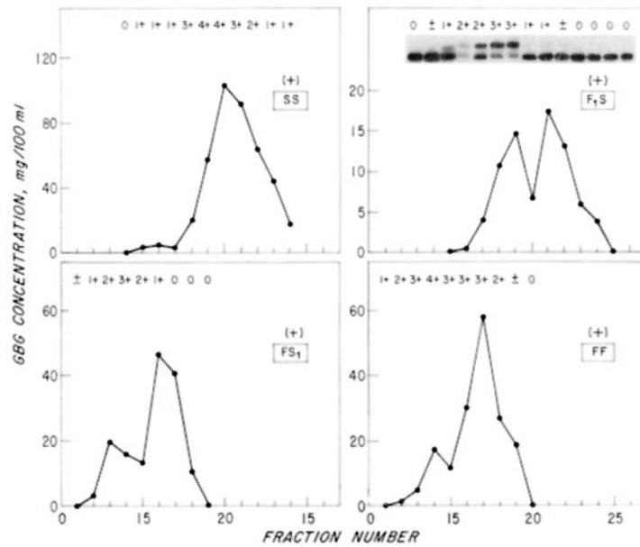
FIG. 3. GBG concentration and serum mediation of CoF inactivation of C 3 in fractions from Pevikon electrophoresis of sera containing different genetic variants of GBG. The anode was at the right in each instance. Gb types of the sera were: SS (upper left), F 1 S (upper right), FS 1 (lower left), and FF (lower right). The distribution of the serum mediator of C 3 inactivation by CoF was assessed by incubating the electrophoretic fractions (in Mg 2+ ) with purified CoF and 125 I-labeled C 3 and subjecting the mixtures to agarose gel electrophoresis and autoradiography. The autoradiographic patterns themselves are shown for Gb F 1 S. Native C 3 is the slower band; inactivation is reflected by conversion to the more rapid band (C 3 i). For this and the remaining sera, C 3 inactivation was graded on a scale of 1-4+, shown above each of the GBG distribution patterns.
