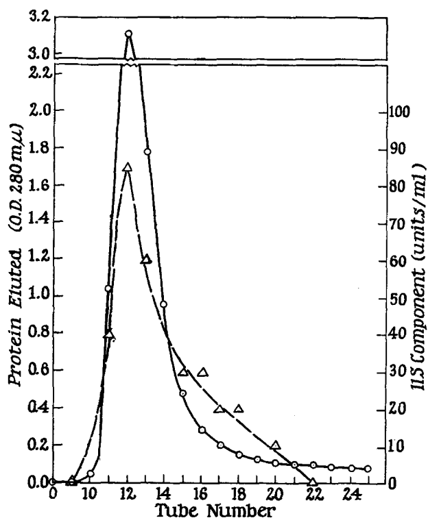
FIG. 5. Identification of C'1q with 11S component: \Delta , 11S component activity; O, protein eluted in the pre- and immediately postgradient area of the chromatogram.
