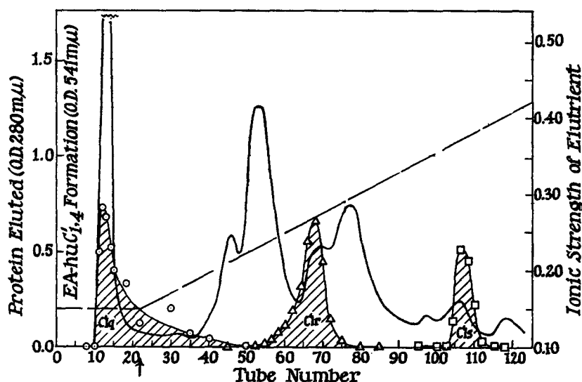
FIG. 2. Chromatographic resolution of C'1 activity of euglobulin fraction into three activities: formation of EA-hu C'1,4 from EA-hu C'4 ; —, protein eluted; — —, ionic strength of elutrient; cross-hatched areas, C'1 activities. The arrow indicates the start of the salt gradient.
