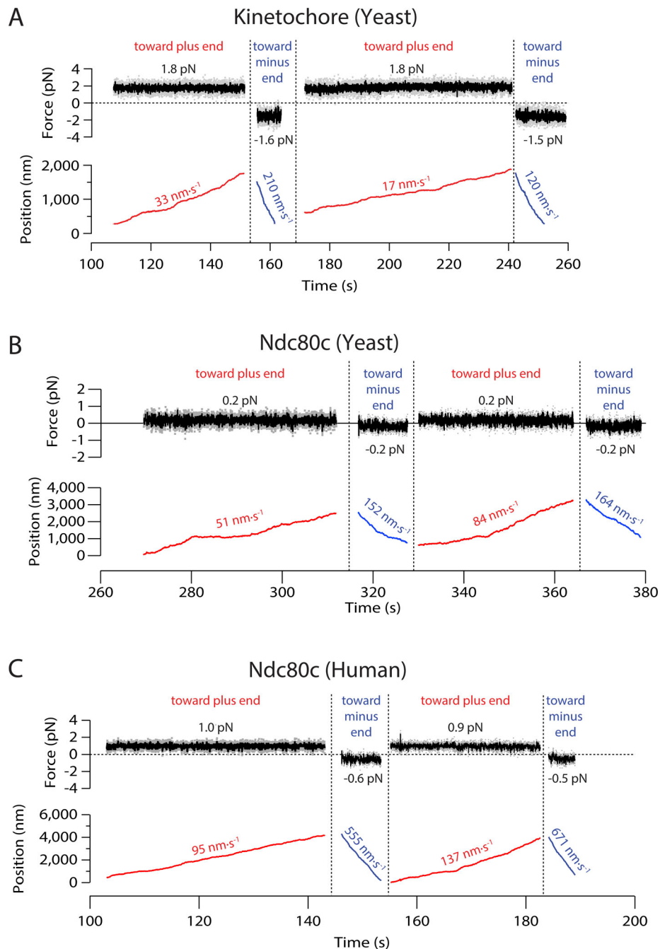
Figure S3. Example records showing measurement of bidirectional sliding friction. (A–C) Force and position are plotted against time for beads decorated with (A) native yeast kinetochore particles, (B) recombinant yeast Ndc80c, or (C) recombinant human Ndc80c, attached to the sides of coverslip-anchored microtubules and pulled alternately toward the plus (red traces) and minus ends (blue traces). Mean forces and speeds for each sliding event are indicated.
