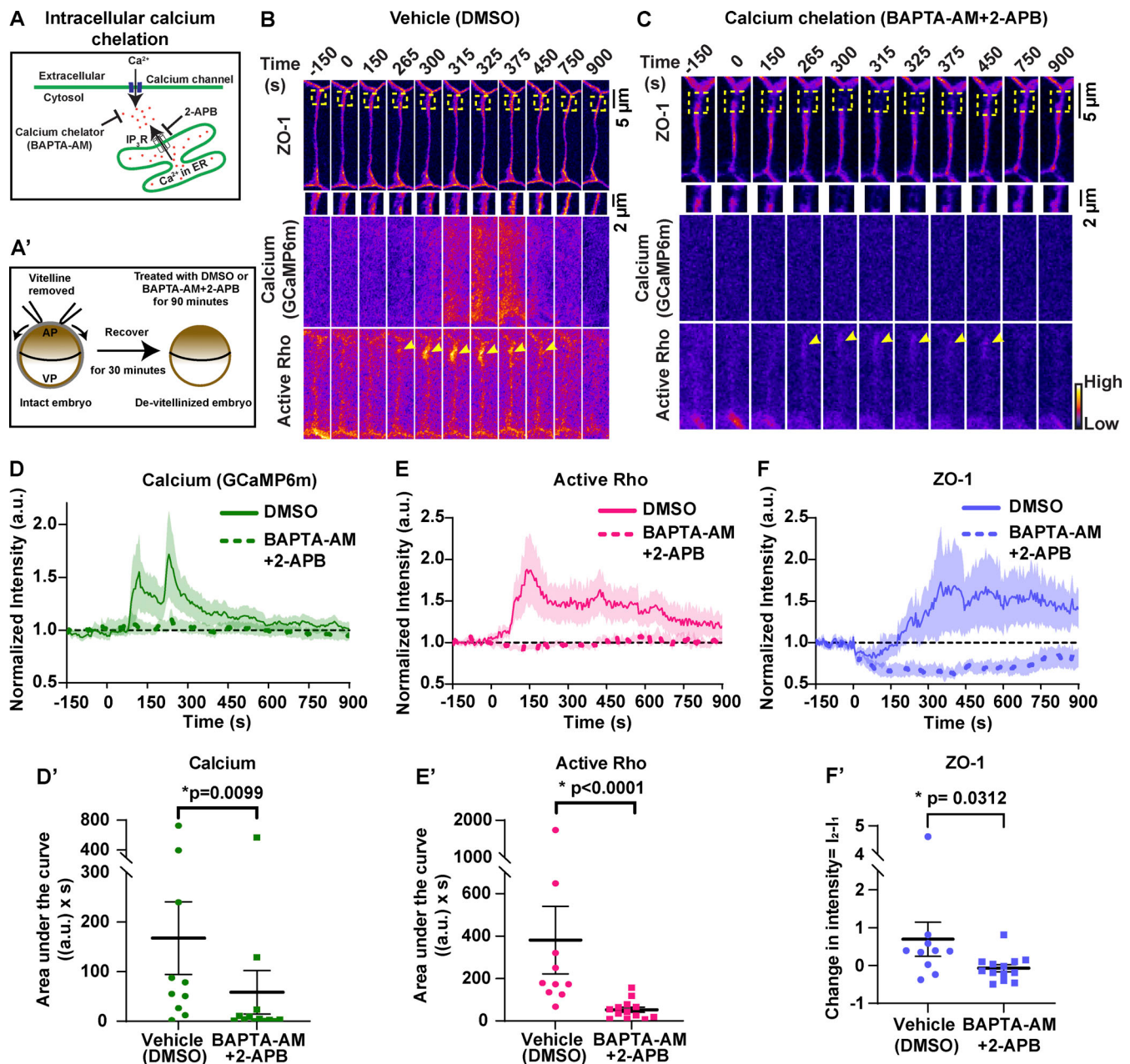
Figure 4. Intracellular calcium flash is required for Rho flare activation and ZO-1 reinforcement. (A) Schematic of cytosolic calcium chelation using BAPTA-AM and blocking \text{IP}_3\text{R} -mediated calcium release from the ER using 2-APB. (A') Schematic showing BAPTA-AM and 2-APB treatment after removal of vitelline envelope. (B and C) Time-lapse images (FIRE LUT) of BFP-ZO-1, calcium (GCaMP6m), and active Rho (mCherry-2xrGBD). Embryos were treated with 0.5% DMSO (vehicle; B) or 20 \mu\text{M} BAPTA-AM and 100 \mu\text{M} 2-APB (calcium chelation; C). Calcium chelation resulted in more severe ZO-1 breaks (yellow boxes, enlarged below) and decreased Rho activity (yellow arrowheads) at the site of ZO-1 loss. Time 0 s represents the start of ZO-1 decrease. (D-F) Graphs of mean normalized intensity of calcium (GCaMP6m; D), active Rho (E), and ZO-1 (F) at the site of ZO-1 loss over time in vehicle (DMSO, solid lines) or calcium chelation (BAPTA-AM + 2-APB, dashed lines) embryos. Shaded region represents SEM. DMSO: n = 10 flares, 7 embryos, 7 experiments; BAPTA-AM + 2-APB: n = 13 flares, 8 embryos, 8 experiments. (D'-F') Area under the curve (AUC) for calcium (D') and active Rho (E') was calculated from D and E, respectively. Scatter plot of change in ZO-1 intensity (F') was calculated from F. I_1 and I_2 represent average intensity of ZO-1 from individual traces from times 0–50 s and 400–450 s, respectively. Error bars represent mean \pm SEM; significance calculated using Mann-Whitney U test.
