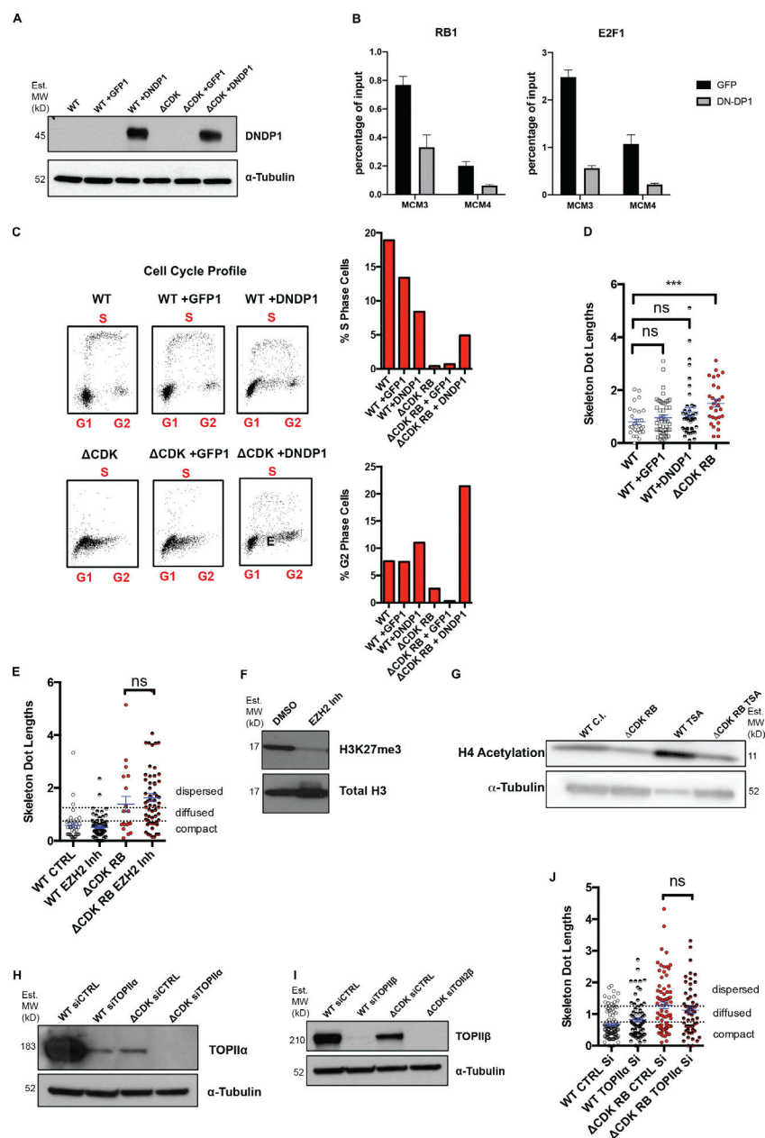
Figure S3. Investigation of the role of DP1, EZH2, HDAC, TOP1 \alpha , and TOP1 \beta in RB-mediated dispersion. (A) Western blots of WT and \Delta CDK-RB RPE cells expressing GFP or DNBP1. MW, molecular weight. (B) E2F ChIP-qPCR and RB1 ChIP-qPCR showing that expression of DNBP1 decreased E2F1 and RB1 binding to sites in the MCM3, MCM4 promoters, compared with cells expressing only GFP. Average scores from three technical replicates were calculated per sample and per epitope. Holm-Sidak multiple t test was performed, and asterisks denote P values. Scale bar = 25 \mu m. (C) Effect of DNBP1 expression on cell cycle profile of the cells in A. Profile shows G1, S, and G2 cells in the different samples. DNBP1 expression in \Delta CDK-RB cells interfered with G1 arrest and increased the percentage of cells in S and G2. (D) Effect of DNBP1 expression on dispersion. Quantitation of mean skeleton dot lengths after DNBP1 expression in WT RPE cells. Expression of DNBP1 in WT RPE does not cause a significant increase in mean skeleton dot length when compared with WT RPE cells or GFP-expressing WT RPE cells. (E) Mean skeleton dot lengths (chromosome 7 \alpha -satellite probe) after WT and \Delta CDK-RB RPE cells were treated with EZH2 inhibitor. (F) Western blot for WT RPE cells treated with DMSO or EZH2 inhibitor (Inh.). Note that treatment with EZH2 inhibitor reduces H3K27 trimethylation levels. (G) Western blot for WT contact inhibited (C.I.) RPE and \Delta CDK-RB treated with TSA for 72 h. H4 acetylation in both WT C.I. and \Delta CDK-RB cells increases after TSA treatment. (H and I) Western blot for WT RPE and \Delta CDK-RB transfected with control and TOP1 \alpha (H) or TOP1 \beta (I) siRNAs. siRNA-mediated knockdown of TOP1 \alpha reduced the levels of the appropriate endogenous protein in WT and \Delta CDK-RB cells. We note that TOP1 \alpha was expressed at lower levels in cells expressing \Delta CDK-RB compared with WT RPE cells. TOP1 \beta siRNA-mediated knockdown causes complete loss of endogenous TOP1 \beta in both WT and \Delta CDK-RB cells. It was also observed that TOP1 \beta levels were lower in \Delta CDK-RB, compared with WT. (J) Mean skeleton dot lengths (chromosome 7 \alpha -satellite probe) after WT and \Delta CDK-RB cells were treated with control and TOP1 \alpha siRNAs. Numbers of foci quantified for each sample (n) are as follows (in the order they appear on the bar graphs): D, n = 29, 48, 40, 29; E, n = 37, 82, 19, 58; J, n = 103, 75, 75, 56. Error bars are SEM. Nonparametric two-tailed Mann-Whitney U test was performed for pairs of samples indicated on graphs, and asterisks denote P values. ns, P > 0.05; ***, P < 0.001. Source data are available for this figure: SourceData FS3. Dashed lines indicate the cutoffs for defining the categories compact, diffused, and dispersed for chromosome 7 \alpha -satellite.
