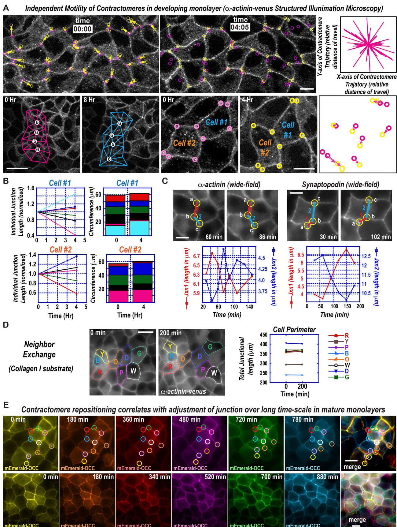
Figure 4. Contractomere motility conserves junctional length. (A) Frames from time-lapse structured-illumination of venus- \alpha -actinin-1 showing contractomere at the beginning (pink circles) and the end (yellow circles) of a 4-h movie. During intercellular organization, junctional length can shorten when
