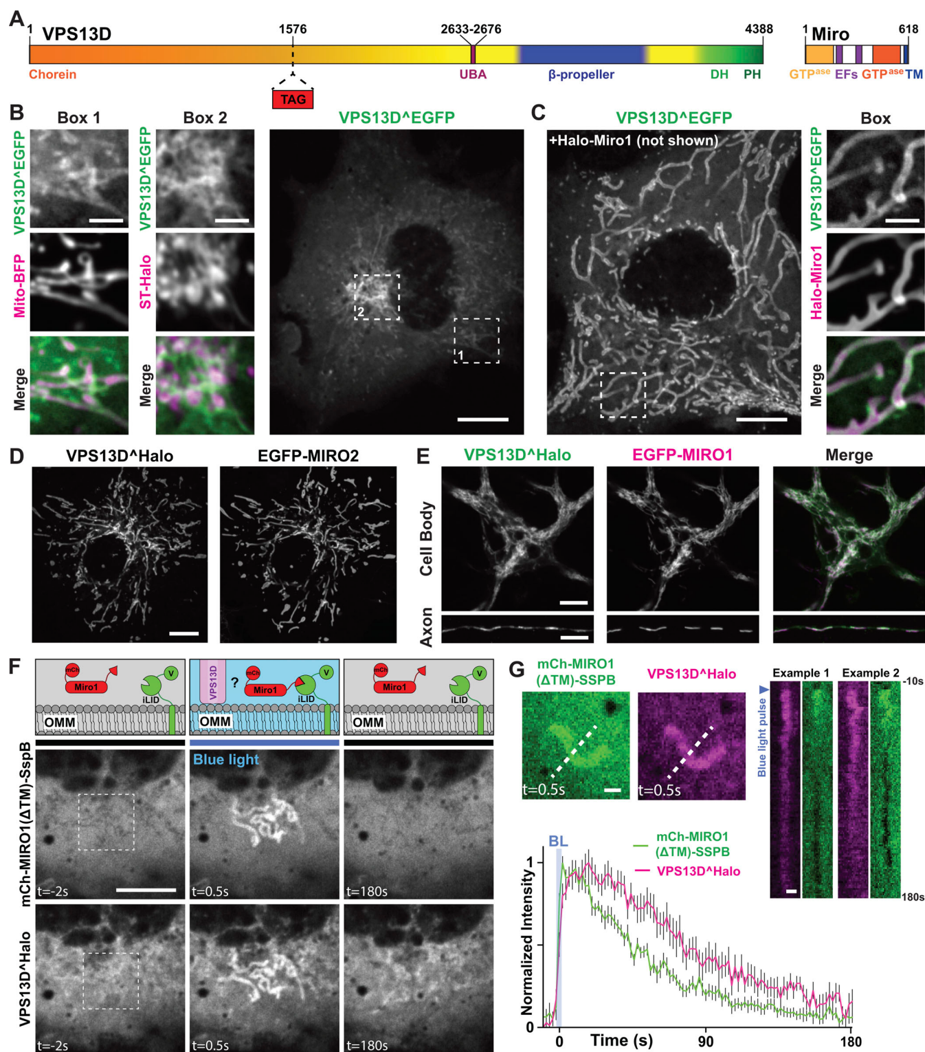
Figure 1. VPS13D recruitment by Miro GTPases. (A) Domain organization of human VPS13D and Miro1. TM, transmembrane. (B) Confocal images of COS7 cell expressing VPS13D Δ EGFP, showing that this protein decorates mitochondria, as shown by colocalization with mito-BFP (Box 1), in addition to being enriched in the Golgi area, visualized by the trans-Golgi marker ST-Halo (Box 2). (C) COS7 cell coexpressing VPS13D Δ EGFP and Halo-Miro1, showing dramatic increase in the localization of VPS13D Δ EGFP to mitochondria produced by Miro overexpression. The region within the white rectangle is shown at higher magnification next to the main field. Fig. 1, B and C, are also shown in Fig. S1, A and C. Scale bars, 10 μm in main panels, 3 μm in insets. (D) Recruitment of VPS13D to mitochondria can also be achieved by coexpression with Miro2. (E) VPS13D Halo and EGFP-Miro1 colocalize in the cell body and processes of a mouse hippocampal neuron. (F) Optogenetic recruitment of the cytosolic domain of Miro1 to the OMM. Top panels: Schematic representation of the experiment, showing that Venus-iLID-Mito in the OMM recruits mCh-Miro1(ΔTM)-SSpB upon blue light excitation. The recruitment of Miro1, in turn, triggers the recruitment of VPS13D. Middle and bottom panels: Confocal images of a COS7 cell show blue light-dependent recruitment and shedding of mCh-Miro1(ΔTM)-SSpB and
