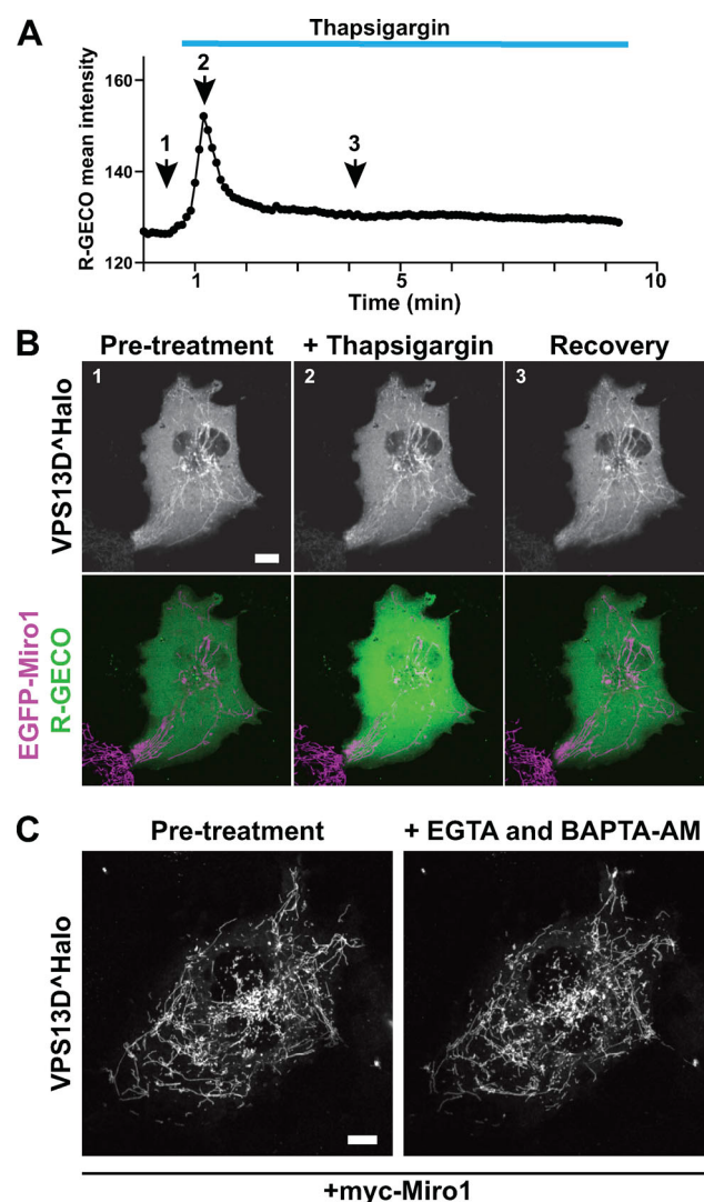
Figure S3. Recruitment of VPS13D to mitochondria by Miro is unaffected by changes in cytosolic \text{Ca}^{2+} . (A and B) COS7 cell expressing EGFP-Miro1, VPS13D Halo and the RFP genetically encoded \text{Ca}^{2+} indicator for optical imaging (R-GECO). (A) Cytosolic \text{Ca}^{2+} levels before and after addition of the sarco/endoplasmic reticulum \text{Ca}^{2+} -ATPase pump inhibitor thapsigargin. (B) Time-lapse confocal images showing snapshot from the time points indicated in A and demonstrating that the localization of VPS13D Halo on mitochondria in the presence of overexpressed Miro1 is not affected by the \text{Ca}^{2+} concentration. (C) Time-lapse confocal images showing that the binding of VPS13D Halo to mitochondria in the presence of coexpressed myc-Miro1 is unaffected by the addition of EGTA and BAPTA-AM to lower intracellular cytosolic \text{Ca}^{2+} . Scale bars, 10 \mu\text{m} .
