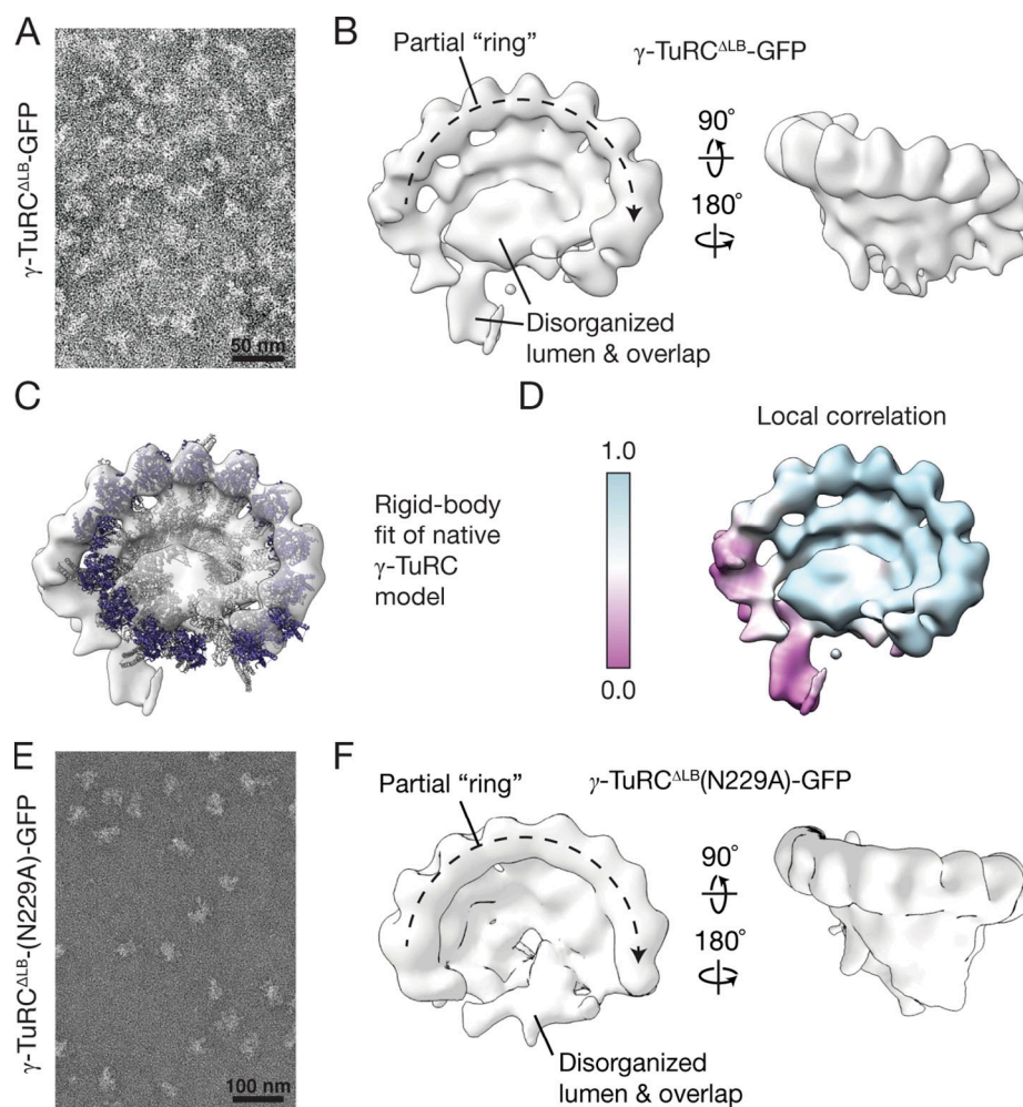
Figure 4. Reconstituted \gamma -TuRC ΔLB -GFP adopts a partial, cone-shaped structure. (A) Transmission EM micrograph of negatively stained \gamma -TuRC ΔLB -GFP. (B) Two views of a 3D reconstruction of \gamma -TuRC ΔLB -GFP from negative-stain EM data. (C) Rigid body fit of the native human \gamma -TuRC model from Fig. 1A into the \gamma -TuRC ΔLB -GFP density map. \gamma -Tubulin molecules are colored in blue; all other subunits are shown in white. Globular densities in the partial ring are numbered. (D) The \gamma -TuRC ΔLB -GFP density map colored according to local correlation of the model fit in C (see Materials and methods). (E) Transmission EM micrograph of negatively stained \gamma -TuRC ΔLB (N229A)-GFP. (F) Two views of a 3D reconstruction of \gamma -TuRC ΔLB (N229A)-GFP from negative-stain EM data.
