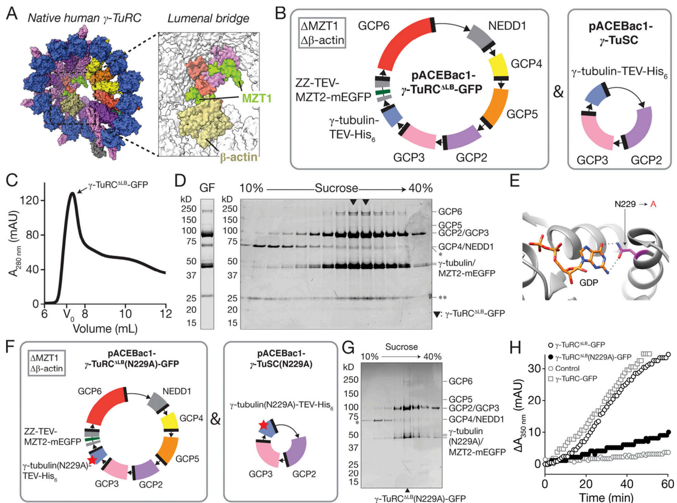
Figure 3. Reconstitution, purification, and functional characterization of \gamma -TuRC ALB -GFP. (A) Surface representation of a model for the native human \gamma -TuRC, as in Fig. 1A. Inset shows the LB and highlights \beta -actin and MZT1. (B) Schematics of recombinant protein constructs used to express \gamma -TuRC ALB -GFP in insect cells. Donor plasmids containing eight \gamma -TuRC ALB -GFP proteins (pACEBac1- \gamma -TuRC ALB -GFP) and \gamma -tubulin-TEV-His 6 /GCP2/GCP3 (pACEBac1- \gamma -TuSC) used to generate bacmids are indicated. (C) Superose 6 elution profile of \gamma -TuRC ALB -GFP IgG eluate. Fractions containing intact \gamma -TuRC ALB -GFP are indicated. The void volume ( V_0 ) of the column was estimated by gel filtering Dextran Blue 2000 in gel filtration buffer. (D) Coomassie-stained SDS-PAGE analysis of \gamma -TuRC ALB -GFP after gel filtration (GF; left) and sucrose gradient centrifugation (right). Solid triangles indicate peak \gamma -TuRC ALB -GFP fractions. Single asterisk indicates an ~70 kD contaminant that does not cosediment with \gamma -TuRC-GFP components. Double asterisk indicates a contaminant at ~25 kD likely to be IgG light chain (Murphy et al., 2001). (E) View of the nucleotide-binding site in the x-ray crystal structure of GDP-bound human \gamma -tubulin (Protein Data Bank accession no. 3CB2; gray cartoon representation). Residue N229 (magenta), which was mutated to alanine in this study, and GDP (colored by element; C and P atoms both colored in orange) are indicated. Predicted hydrogen bonds formed between N229 and the guanine moiety of GDP are shown (dotted black lines). (F) Schematics of the recombinant protein constructs used to express \gamma -TuRC ALB (N229A)-GFP in insect cells. Donor plasmids containing the eight \gamma -TuRC ALB (N229A)-GFP proteins (pACEBac1- \gamma -TuRC ALB (N229A)-GFP; left) and \gamma -tubulin(N229A)-TEV-His 6 /GCP2/GCP3 (pACEBac1- \gamma -TuSC[N229A]; right) are indicated. The N229A point mutation is highlighted by a red star in the \gamma -tubulin(N229A) coding fragments. Coding fragments are colored as in Fig. 1A. (G) Coomassie-stained SDS-PAGE analysis of \gamma -TuRC ALB (N229A)-GFP sucrose gradient centrifugation fractions. Asterisk indicates an ~70 kD contaminant that does not cosediment with \gamma -TuRC ALB (N229A)-GFP components. Peak \gamma -TuRC ALB (N229A)-GFP fraction is indicated by a solid triangle at the bottom of the gel. Note: Only odd-numbered gradient fractions were run on this particular gel. (H) Turbidity-based microtubule nucleation assay of reactions containing tubulin (20 \mu M) and GTP (1 mM) alone (hollow gray circles), in the presence of 0.25 nM \gamma -TuRC ALB -GFP (hollow black circles), or in the presence of 0.25 nM \gamma -TuRC ALB (N229A)-GFP (solid black circles). Turbidity data for \gamma -TuRC-GFP from Fig. 1D (gray squares) are also shown for comparison.
