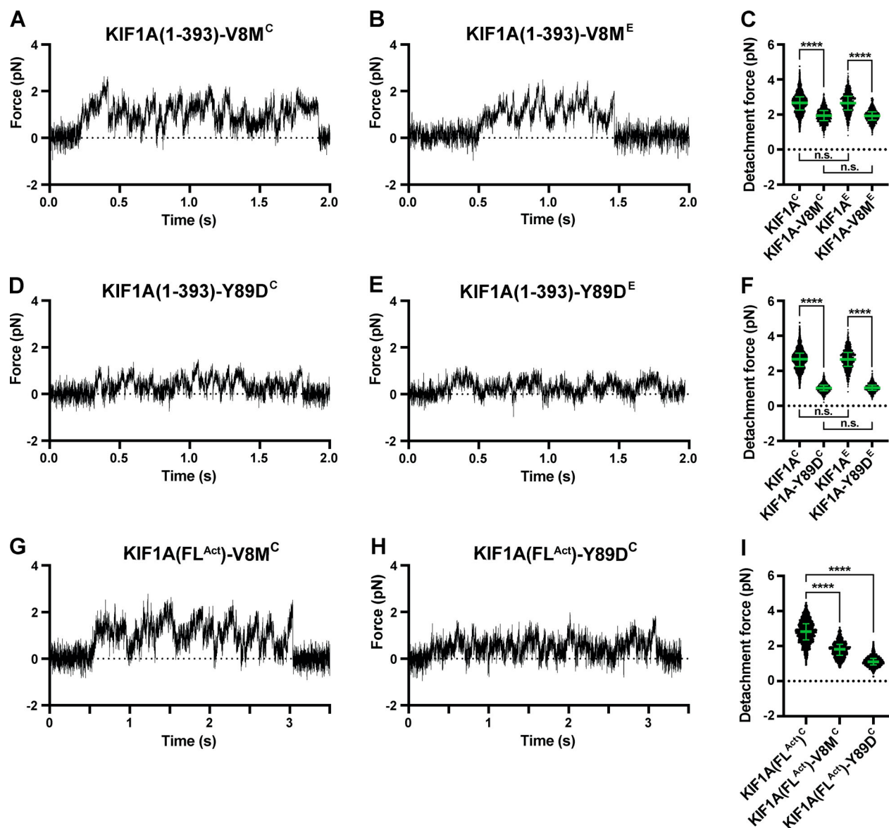
Figure 7. V8M and Y89D mutations result in decreased force output for KIF1A motors. (A, B, D, and E) Representative force versus time records of bead movement driven by single molecules of KIF1A(1-393)-V8M C (A), KIF1A(1-393)-V8M E (B), KIF1A(1-393)-Y89D C (D), or KIF1A(1-393)-Y89D E (E). k = 0.04 – 0.05 pN/nm. (C) Detachment forces of KIF1A(1-393) C ( 2.66 [2.25, 3.01] pN, n = 1,912 ), KIF1A(1-393)-V8M C ( 1.94 [1.65, 2.22] pN, n = 1,343 ), KIF1A(1-393) E ( 2.65 [2.25, 3.05] pN, n = 1,044 ), and KIF1A(1-393)-V8M E ( 1.92 [1.68, 2.15] pN, n = 1,032 ). Statistical significance was determined using an unpaired Welch's t test (****, P < 0.0001 ). (F) As in C, but for KIF1A(1-393)-Y89D C ( 1.02 [0.87, 1.19] pN, n = 1,468 ) and KIF1A(1-393)-Y89D E ( 1.03 [0.89, 1.19] pN, n = 1,213 ). (G and H) As in A, but for KIF1A(FL Act )-V8M C (G) and KIF1A(FL Act )-Y89D C (H). k = 0.04 – 0.05 pN/nm. (I) As in C, but for KIF1A(FL Act ) C ( 2.82 [2.35, 3.27] pN, n = 1,433 ), KIF1A(FL Act )-V8M C ( 1.81 [1.48, 2.10] pN, n = 1,024 ) and KIF1A(FL Act )-Y89D C ( 1.10 [0.92, 1.29] pN, n = 1,022 ). Data were analyzed across two or three independent experiments. Green bars in C, F, and I indicate the median values with quartiles. n.s., not significant.
