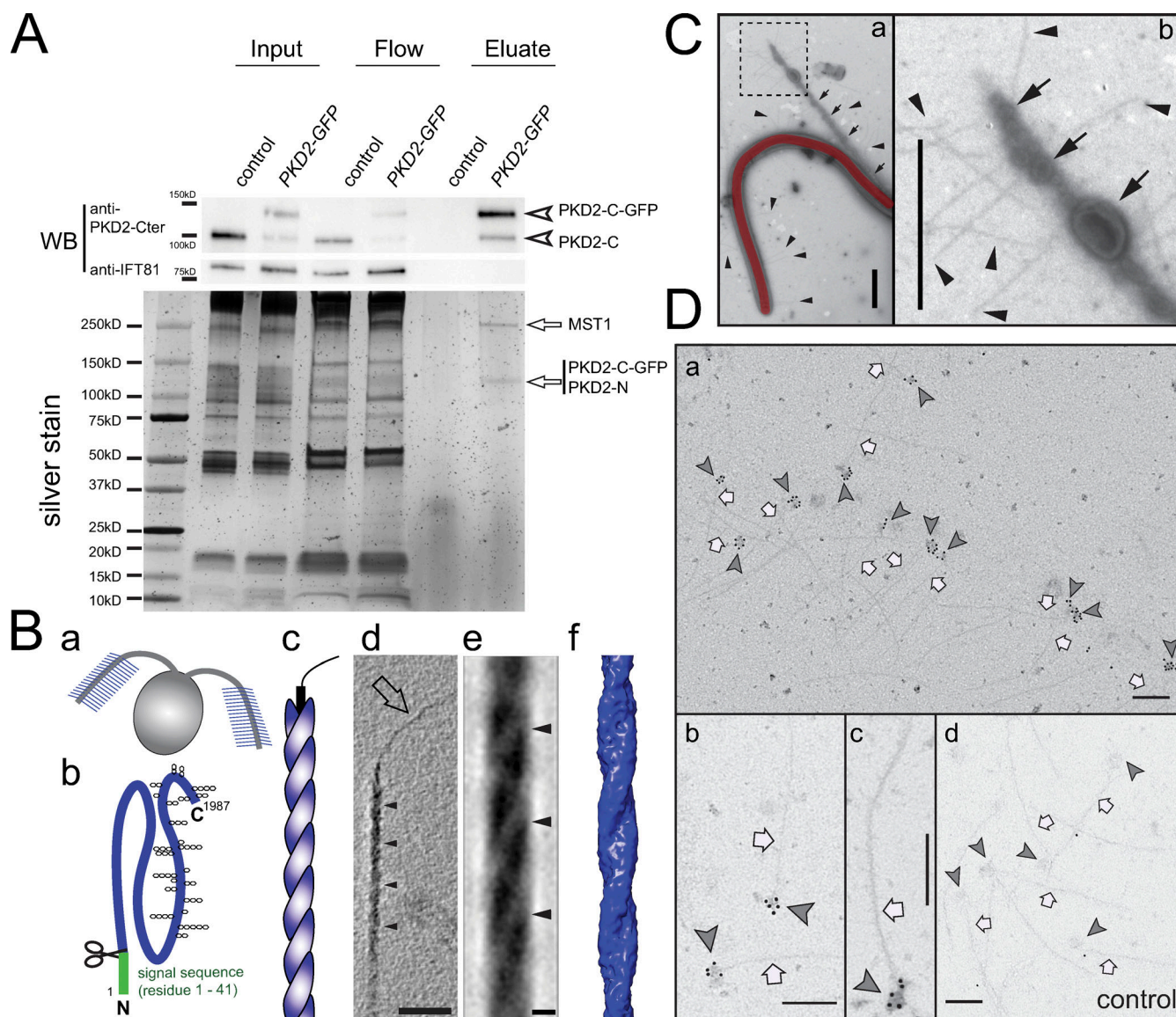
Figure 3. PKD2 binds to the mastigoneme protein MST1. (A) PKD2-GFP pull-down assay using a wild-type control strain ( gl1 ) and a strain expressing both endogenous and GFP-tagged PKD2. Shown are the detergent extracts of isolated cilia (Input), the flow-throughs, and the eluates from the anti-GFP nanobody trap. Top: Western blot (WB) showing pull-down of both the GFP-tagged and the endogenous C-terminal fragment of PKD2 indicating PKD2 oligomers. Antibodies to IFT81 were used as loading control. Bottom: Silver-stained SDS-PAGE. Mass spectrometry identified the bands marked by arrows as MST1 and a mix of the PKD2-C-GFP and PKD2-N. (Ba–Bc) Schematic representation of Chlamydomonas with mastigonemes in blue (a), MST1 with the predicted signal sequence in green (b; trapezoids indicate glycosylation), and a single mastigoneme (c). (Bd) 20-nm-thick tomographic slice of a mastigoneme showing the periodic substructure (arrowheads) of the main filament and the thinner extended tip (arrow). Bar = 50 nm. (Be and Bf) 1-nm-thick tomographic slice (e) and a full-volume 3D isosurface rendering representation (f) of the subtomogram average based on 1,977 repeat units from 73 mastigonemes after applying fourfold symmetry. Bar = 5 nm. (C) Whole-mount negative stain of an intact Chlamydomonas wild-type cilium. Mastigonemes (arrowheads), released vesicle-like structures (arrows), and cilium (colored in red) are marked in panel a. Enlarged image of the boxed area in panel a showing the vesicle-like structures and mastigonemes (b). Bar = 500 nm. (D) Anti-GFP whole-mount immunogold staining of mastigonemes released from pkd2 PKD2-GFP cells (a–c) and control cilia (d). 10-nm gold complexes decorate the base (arrowheads) of many mastigonemes (arrows) of the PKD2-GFP strain. Bars = 200 nm.
