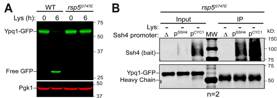
Figure S3. ColP of Ypq1 and Ssh4 in the presence of an Rsp5 mutant. Related to Fig. 2. (A) Degradation of Ypq1-GFP before (0 h) or after (6 h) Lys starvation in the presence of WT Rsp5 or rsp5 G747E . (B) ColP of Ypq1-GFP with WT Ssh4 (bait) expressed under its native promoter (p Ssh4 ) or an overexpression promoter (p CYC1 ) in a weak Rsp5 mutant ( rsp5 G747E ) background. IP, immunoprecipitation.
