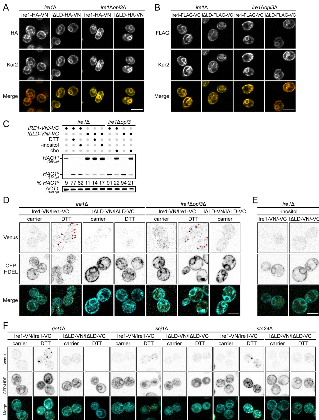
Figure S3. Ire1 clusters are mostly driven by DTT-induced proteotoxic stress. (A and B) Cells were grown to early log phase in selective synthetic complete media before being fixed in formaldehyde and permeabilized. Staining was performed using anti-HA (A) or anti-FLAG (B) and anti-Kar2 primary antibodies. Scale bar, 5 \mu m. (C) RT-PCR of unspliced HAC1 ( HAC1 U ) and spliced ( HAC1 S ) mRNA. Media was depleted of inositol (-inositol), supplemented with 1 mM choline (cho) or incubated 1 h with 1 mM DTT, when indicated. Actin ( ACT1 ) was used as loading control. (D and E) Cells coexpressing the pair of split Venus fragments to monitor IRE1-HA-VN173 and IRE1-FLAG-VC155 or IRE1ΔLD-HA-VN173 and IRE1ΔLD-FLAG-VC155 to dimerization in vivo by BiFC in ire1Δ and ire1Δopi3Δ . Cells were treated 1 h with 10 mM DTT (D) or depleted of inositol (-inositol; E), when indicated. CFP-HDEL was used as ER marker. Red arrowheads indicate Ire1 puncta. (F) Mutant strains get1Δ , scj1Δ , and ste24Δ treated as in D.
