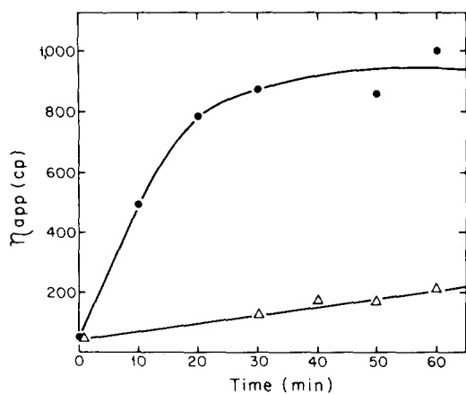
FIGURE 4 Increase in viscosity as a function of time. Low-salt washed lysosomal membrane (1 mg/ml) was mixed with actin (0.8 mg/ml) in polymerization buffer described under Materials and Methods. Samples were incubated at room temperature for the indicated period of time and assayed. ●, low-salt washed lysosomal membrane with actin; Δ, actin alone.
