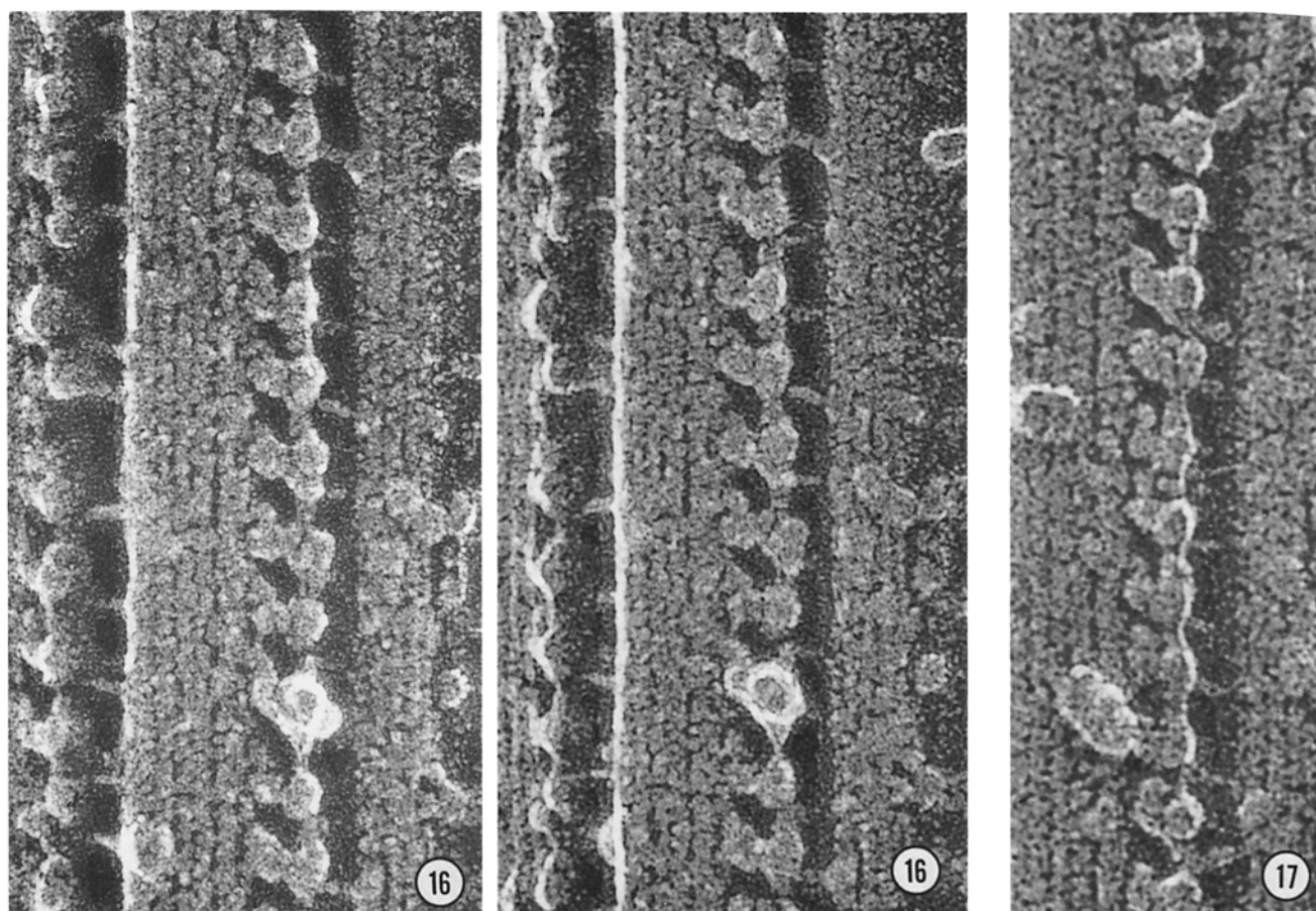
FIGURES 16 and 17 Fig. 16. Relaxed Chlamydomonas axoneme, unfixed, incubated in 0.2 mM vanadate and then 1 mM ATP. Stereo pair. Head-to-head linkers are seen to advantage. \times 480,000 . Fig. 17. Relaxed Chlamydomonas axoneme, unfixed, incubated in 1 mM ATP. Note how this "ATP image" is indistinguishable from the "vanadate image" of Fig. 16. \times 480,000 .
