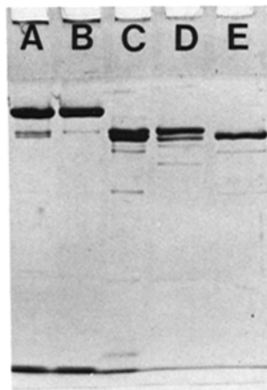
FIGURE 3 SDS PAGE (7.5% acrylamide) of the fractions obtained during the purification of PLD C-protein. Lane A: Crude PLD myosin before DEAE-Sephadex chromatography (2.5 µg). Lane B: PLD myosin after DEAE-Sephadex chromatography (2.3 µg). Lane C: Crude C-protein before HA chromatography (2.1 µg). Lane D: First peak from HA column (1.4 µg). Lane E: Second peak of the HA column (1.2 µg).
