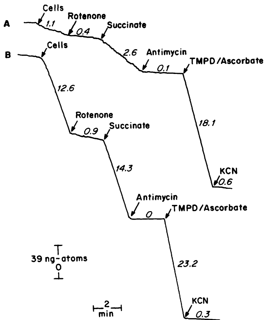
FIGURE 2 Addition of mitochondrial substrates to CM-injured L1210 cells permeabilized with digitonin. Top: A simplified scheme of the respiratory chain with sites of action of some mitochondrial inhibitors is shown for reference. Trace A: L1210 cells following an 18-h incubation with CM. Trace B: Uninjured L1210 cells. Respiration medium contained 5.0 mM malate and cells were permeabilized with 0.005% digitonin. Substrates and inhibitors were added at the final concentrations given in Table I. KCN was 1.0 mM. Traces were made with \sim 5 \times 10^6 cells per ml. The reaction vessel contained 1.2 ml. Numbers are rates of oxygen consumption in nanogram atoms per minute per 10^6 L1210 cells.
