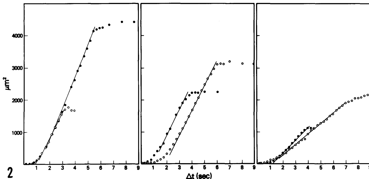
FIGURE 2 Plots of (length of the acrosomal process) 2 in square micrometers as a function of time in seconds after the process first becomes visible. Of note is that, except for the beginning and very end of the reaction, the points fall exactly on a straight line. In the left hand curve sperm B (closed circles) and J (open circles) are illustrated; in the middle, we see sperm D (closed circles) and C (open circles); and in the right hand graph, sperm F (closed circles) and A (open circles) are seen.
