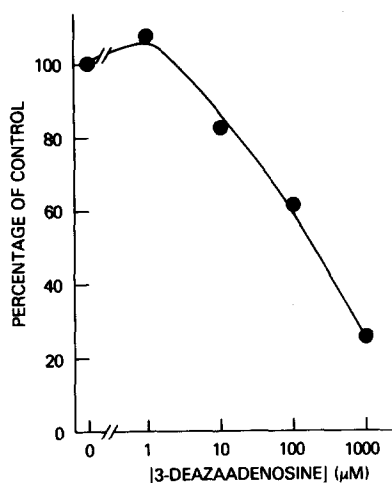
FIGURE 4 Dose-response curve for inhibition of fMet-Leu-Phe-stimulated [ 14 C]arachidonic acid release by 3-deazaadenosine. Neutrophils were preincubated with arachidonic acid for 30 min at 37°C, washed, and preincubated with various concentrations of 3-deazaadenosine and 100 μM homocysteine for 30 min at 37°C before stimulating for 5 min with 10 nM fMet-Leu-Phe. Results are expressed as means of triplicate determinations. Uninhibited release was 480% over unstimulated samples (stimulated release = 3,080 DPM/5 × 10 6 cells; unstimulated release = 645 DPM/5 × 10 6 cells). Abscissa is logarithmic.
