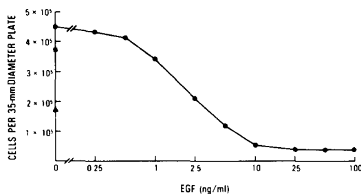
FIGURE 3 Concentration dependence of EGF inhibition of A431 cell growth. Cells were counted after incubation for 6 d in plates containing F12:DME+4F with the indicated concentrations of EGF (●—●); F12:DME (▲); F12:DME+FCS (■).
