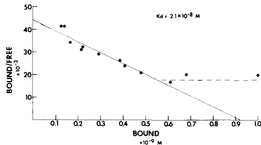
FIGURE 8 Scatchard plot of binding of f-NorleuLeuPhe to rabbit PMNs. Cells were incubated for 20 min at 4^{\circ}\text{C} in various concentrations of [ ^3\text{H} ]f-NorleuLeuPhe. The peptide bound was determined from the cell-associated counts which remain on the glass filter; the free peptide was determined by counting an aliquot of the measured filtrate plus wash. The line was drawn by a linear regression equation, omitting the two points with the highest binding. The coefficient r for the line is -0.96 .
