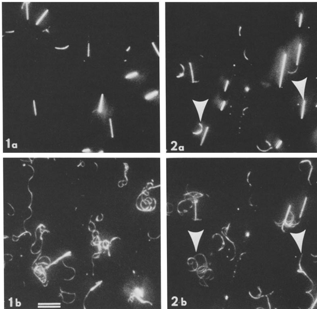
FIGURES 1 and 2 Dark-field light micrographs of trypsin-treated axonemes before (Figs. 1 a and 2 a ) and after (Figs. 1 b and 2 b ) addition of 0.2 mM ATP. Axonemes were photographed while attached to the coverglass. Bar, 20 \mu M. \times 470.
