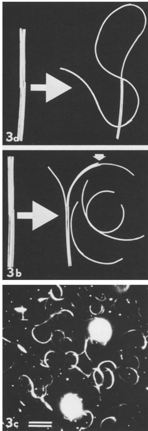
FIGURE 3 (a) Model of ATP-induced sliding disruption of ^{80}\text{S} axonemes suspended in buffer. (b) Model of ATP-induced peeling disruption of a vanadate-treated ^{80}\text{S} axoneme suspended in buffer. (c) Examples of the C-shaped structures, presumably single or small groups of doublet microtubules, resulting from ATP-induced disruption of a suspension of vanadate-treated ^{80}\text{S} axonemes.
