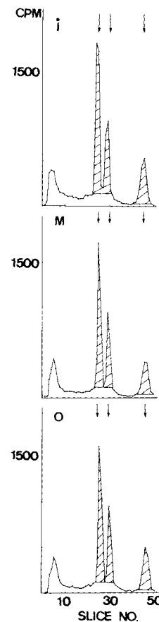
FIGURE 1 Electrophoretic separations in 1.5% agarose of the RNA from cytoplasmic zones of 12 cells isolated from the salivary gland of an animal that was injected with 25 \mu Ci of tritiated uridine 18 h before sacrifice. Arrows denote, from left to right, the positions of 23 S, 16 S, and 4 S RNA, added markers of RNA from E. coli . The letters i , m , o stand for inner, middle, and outer cytoplasmic zones.
