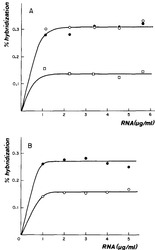
FIGURE 1 Saturation hybridization experiments between R. americana rRNA and DNA obtained from several R. americana tissues and organs. Preparations of ovary and carcass DNA from adult females, and of fat body and salivary gland DNA from third period larvae were denatured by alkali, immobilized on nitrocellulose filters (about 10 \mu\text{g} DNA/filter) and hybridized with increasing amounts of 28S + 18S [ 3 H]rRNA (42,000 cpm/ \mu\text{g} ), as described in Materials and Methods. The radioactivity was determined in a liquid scintillation spectrometer model L 250 (Beckman Instruments). The mean background of radioactivity measured 0.1% of the total radioactivity in the reaction tubes. DNA retention averaged 97% of the DNA input. Fig. 1 A ●—● ovary DNA; ○—○ carcass DNA; □—□ gland DNA. Fig. 1 B ●—● fat body DNA; ○—○ gland DNA.
