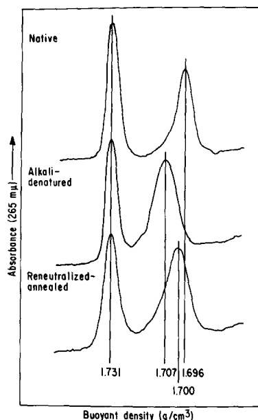
FIGURE 2 Densitometer tracings of ultraviolet photographs of cesium chloride equilibrium density gradients of S. oleracea chloroplast DNA after the treatments indicated. The reference band ( \rho = 1.731 \text{ g/cm}^3 ) to the left is native DNA of M. lysodeikticus .
