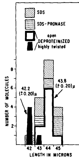
FIGURE 5 Frequency distribution of the lengths of circular DNA molecules from a chloroplast fraction of S. oleracea . The DNA was prepared directly for electron microscopy after the treatments indicated. The mean and standard error on the left are for the supercoiled molecules from the deproteinized sample. The mean and standard error on the right are for the remaining molecules, which are all open and which represent five molecules from the SDS lysate, five from the SDS-pronase digest, and 10 from the deproteinized DNA preparation.
