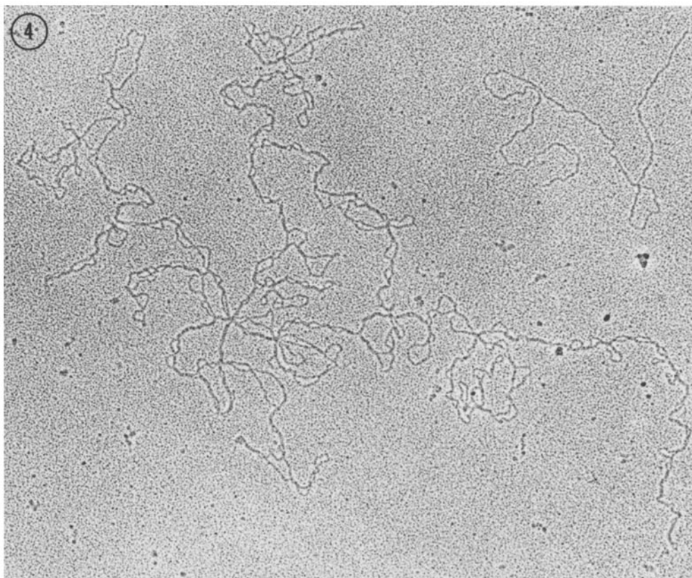
FIGURE 4 Electron micrograph of a rotary-shadowed highly twisted circular molecule of DNA from a deproteinized preparation of chloroplasts of S. oleracea . The molecule is 42 \mu in total length. \times 43,300 .
