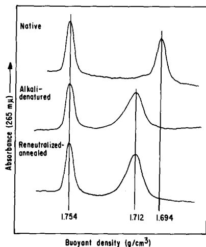
FIGURE 1 Densitometer tracings of ultraviolet photographs of cesium chloride equilibrium density gradients of S. oleracea whole cell DNA after the treatments indicated. The reference band ( \rho = 1.754 \text{ g/cm}^3 ) to the left is E. coli bromouracil-labeled hybrid DNA.
