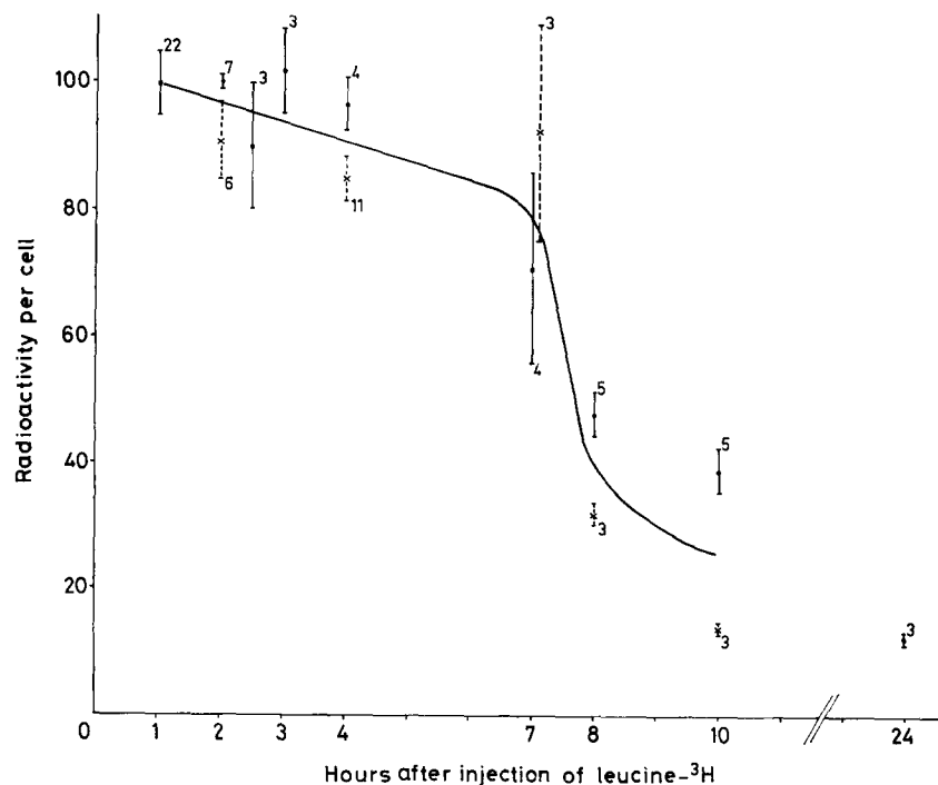
FIGURE 2 Loss of radioactive protein per cell in the rat pancreas during continued fasting after injection of leucine- 3 H. Means \pm SEM; number of animals mentioned for each point. ●, series I (100% = 9.0 silver grains per mean cellular area); ×, series II (100% = 15.1 silver grains per mean cellular area).
