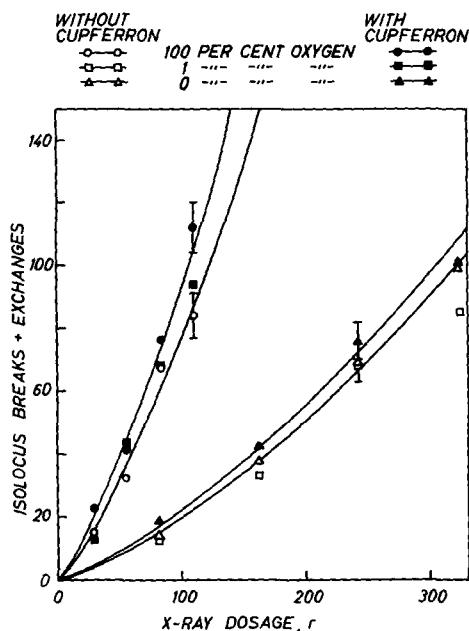
FIG. 5. The relation between the x-ray dosage and the frequencies of isolocus breaks + exchanges induced in the presence and absence of cupferron ( 400 \mu\text{M/liter} ) and with 0, 1, and 100 per cent oxygen in the gas.
