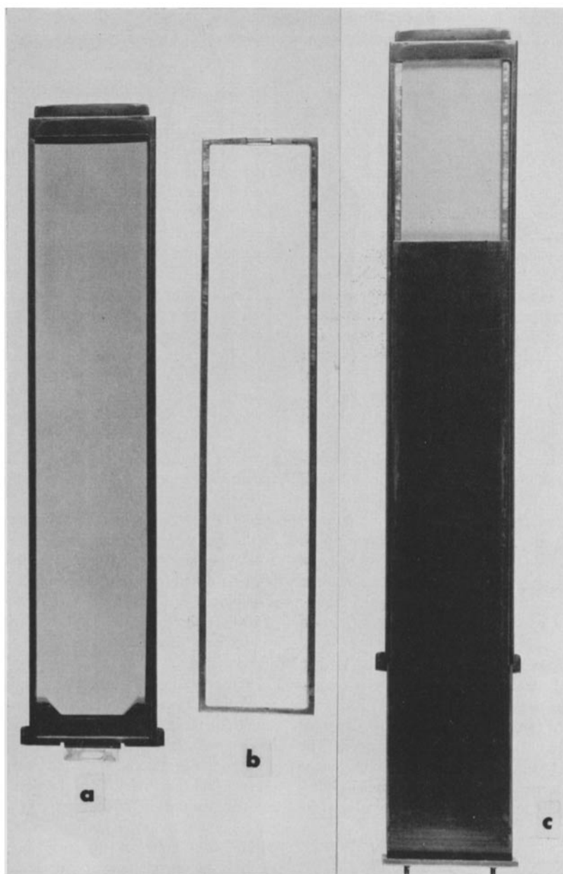
FIG. 1 a . RCA-EMU-2 film cassette holding 2 \times 10 strip of fine grain positive sheet film. Cassette cover removed. No brass retaining frame. b . Brass retaining frame for holding sheet film strip in position in cassette. c . Film cassette with sheet film strip and retaining frame in position. Cassette cover partially closed.
