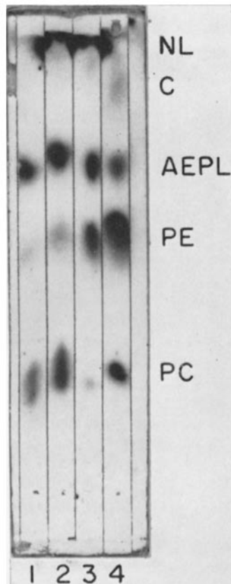
FIGURE 7 Thin-layer chromatogram developed in chloroform:acetic acid:methanol:water (75:25:5:2.2). 1, Cilia; 2, Ciliary supernatant; 3, Pellicle; 4, Mitochondria. PC , choline phosphatides (+ lyso PE); PE , ethanolamine phosphatides; AEPL , 2-aminoethylphosphonate lipids; C , cardiolipin; NL , neutral lipids.
