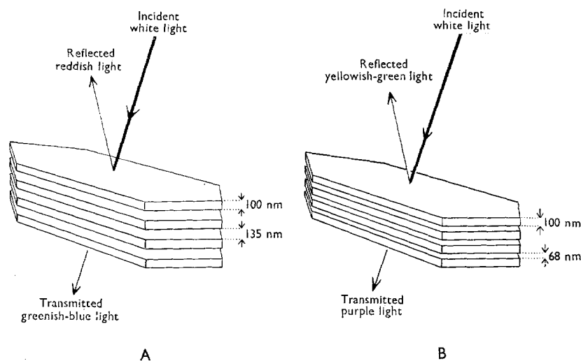
FIGURE 1 (A) Diagram of a platelet showing a stack of crystals of thickness and spacing to give the best reflexion for light of 720 nm. The thickness of the crystals and their spacing is relatively exaggerated. A typical platelet from a scale of a sprat would have a broad surface of about 25 \mu\text{m} \times 5 \mu\text{m} , and the whole stack of crystals and spaces would be about 1 \mu\text{m} thick. Platelets of this kind are shown in cross-section in Fig. 2 C. (B) The same platelet as that shown in (A) but the distances between the crystals have been halved and therefore the wave bands of light reflected and transmitted have been very greatly changed. The wave band best reflected is now around 540 nm.
