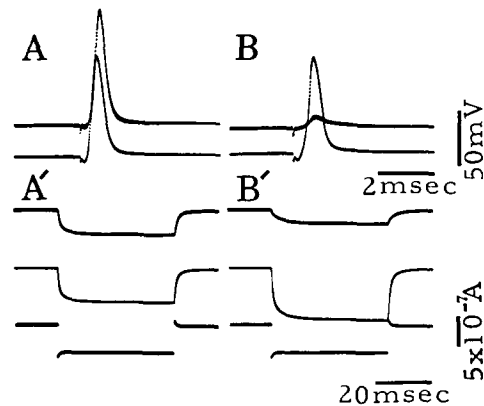
FIGURE 3 Effect of mechanical injury on coupling at the septum. A and A' , records before injury; B and B' , records 60 min after cutting through the rostral axon with scissors. In each record the upper trace shows the potential in the rostral segment, and the second trace shows the potential in the caudal segment. Propagated spikes in A and B were evoked by stimulation of the caudal axon; in B , only a small postjunctional potential was recorded in the rostral segment. An equal hyperpolarizing pulse was applied on the caudal side in A' and B' (3rd traces). The resulting potential was larger on the caudal side and smaller on the rostral side after injury.
