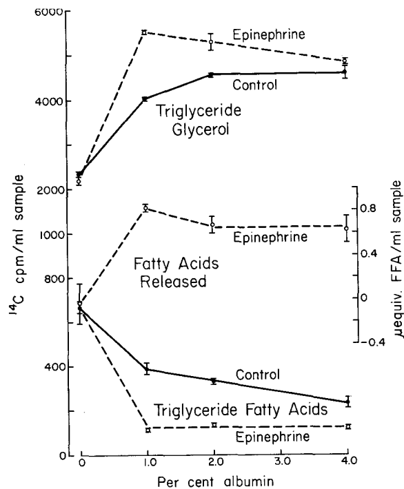
FIGURE 5 Triglyceride glycerol- 14 C and triglyceride fatty acid- 14 C production in the presence of 0.1 \mu g epinephrine per ml or in the absence of hormones and nonesterified fatty acid (FFA) release in the presence of 0.1 \mu g epinephrine per ml versus serum albumin concentration. Isolated adipose cells incubated 60 min in the presence of 0.1 mg glucose per ml.
