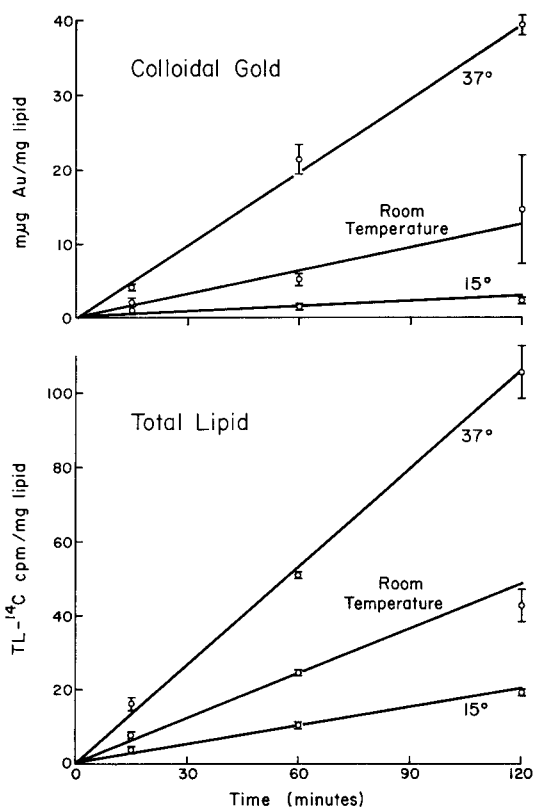
FIGURE 3 Colloidal gold uptake and total lipid (TL)- ^{14}\text{C} production versus time at 15°C, room temperature, and 37°C. Isolated adipose cells incubated in KRB-albumin buffer in the presence of 100 \mu\text{g} colloidal gold and 1.6 mg glucose per ml and in the absence of hormones.
