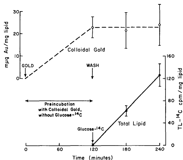
FIGURE 4 Release of colloidal gold taken up and total lipid (TL)- 14 C production versus time. Isolated adipose cells incubated in KRB-albumin buffer in the presence of 10 \mu g colloidal gold and 1.0 mg glucose per ml and in the absence of hormones; reincubated in KRB-albumin buffer in the presence of 1.0 mg glucose per ml and in the absence of colloidal gold and hormones.
