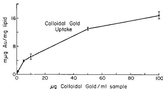
FIGURE 2 Colloidal gold uptake versus colloidal gold concentration. Isolated adipose cells incubated 60 min in KRB-albumin buffer in the absence of hormones. Values \pm standard deviation.
