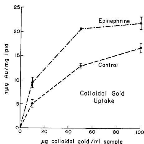
FIGURE 8 Colloidal gold uptake versus colloidal gold concentration in the presence of 10 \mu\text{g} epinephrine per ml or in the absence of hormones. Isolated adipose cells incubated 60 min in KRB-albumin buffer.
