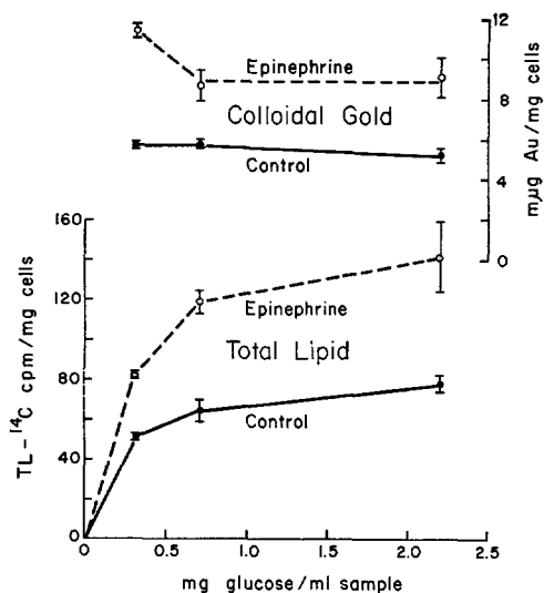
FIGURE 11 Colloidal gold uptake and total lipid (TL)- 14 C production versus glucose concentration in the presence of 1.0 \mu g epinephrine per ml and in the absence of hormones. Isolated adipose cells incubated 60 min in KRB-albumin buffer in the presence of 10 \mu g colloidal gold per ml.
