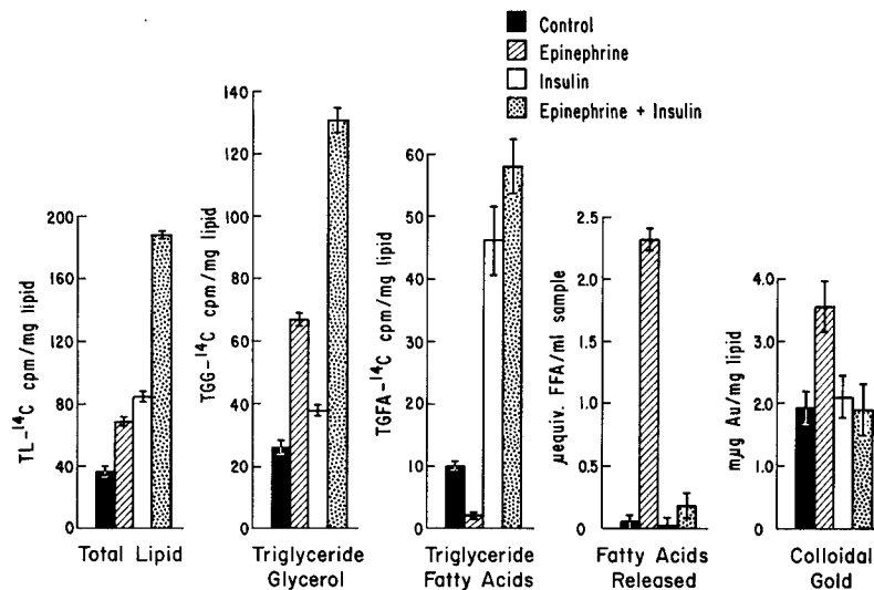
FIGURE 13 Total lipid ( TL )- ^{14}C , triglyceride glycerol ( TGG )- ^{14}C , and triglyceride fatty acid ( TGFA )- ^{14}C production, nonesterified fatty acid ( FFA ) release, and colloidal gold uptake in the presence of 1.0 \mu g epinephrine, 100 \mu U insulin, or 1.0 \mu g epinephrine plus 100 \mu U insulin per ml or in the absence of hormones. Isolated adipose cells incubated 60 min in KRB-albumin buffer in the presence of 0.35 mg glucose and 10 \mu g colloidal gold per ml.
