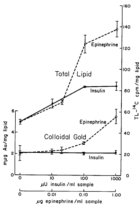
FIGURE 7 Colloidal gold uptake and total lipid ( TL )- ^{14}C production versus insulin and epinephrine concentration. Isolated adipose cells incubated 60 min in KRB-albumin buffer in the presence of 10 \mu\text{g} colloidal gold and 0.75 \text{ mg} glucose per ml.
