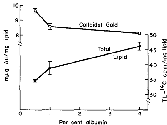
FIGURE 5 Colloidal gold uptake and total lipid (TL)- 14 C production versus serum albumin concentration. Isolated adipose cells incubated 60 min in KRB buffer in the presence of 10 \mu g colloidal gold and 1.28 mg glucose per ml and in the absence of hormones.
