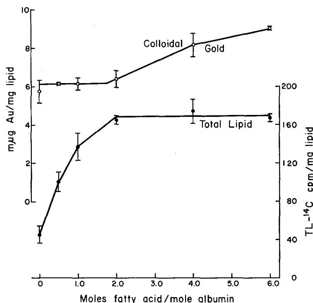
FIGURE 6 Colloidal gold uptake and total lipid (TL)- ^{14}\text{C} production versus fatty acid to albumin molar ratio. Isolated adipose cells incubated 60 min in KRB-albumin buffer in the presence of 10\ \mu\text{g} colloidal gold and 0.98\ \text{mg} glucose per ml and in the absence of hormones.
