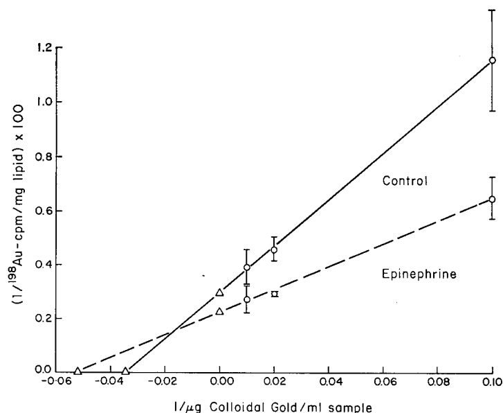
FIGURE 9 Reciprocal of colloidal gold uptake versus reciprocal of colloidal gold concentration in the incubation medium in the presence of 10 \mu\text{g} epinephrine per ml or in the absence of hormones. Isolated adipose cells incubated 60 min in KRB-albumin buffer. \circ , experimental point; \triangle , calculated point.
