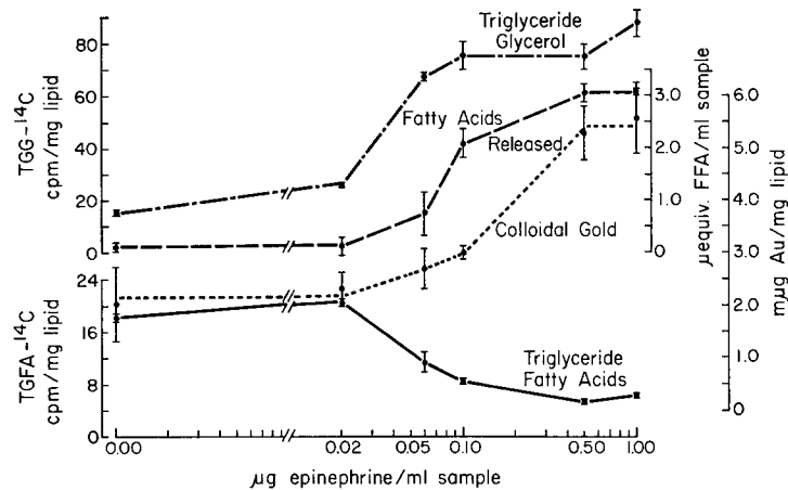
FIGURE 12 Triglyceride glycerol ( TGG )- ^{14}C and triglyceride fatty acid ( FFA ) ( TGFA )- ^{14}C production, colloidal gold uptake, and nonesterified fatty acid release versus epinephrine concentration. Isolated adipose cells incubated 60 min in KRB-albumin buffer in the presence of 1.28 mg glucose and 10 \mu g colloidal gold per ml.
