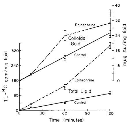
FIGURE 10 Colloidal gold uptake and total lipid (TL)- ^{14}\text{C} production versus time in the presence of 10 \mu\text{g} epinephrine per ml or in the absence of hormones. Isolated adipose cells incubated in KRB-albumin buffer in the presence of 35 \mu\text{g} colloidal gold per ml.
