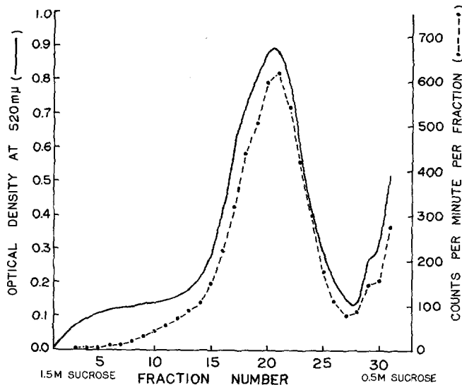
FIGURE 2 Velocity sedimentation of normal rat liver mitochondria from animals which had previously received 100 \mu Ci of leucine- ^{14} C (preparation (c) under Methods). After centrifugation for 75 min in a linear 0.5–1.5 M sucrose density gradient the optical density at 520 m \mu and radioactivity of the effluent from the gradient were monitored as described under Methods. The positions of the optical density (solid line) and radioactivity (dashed line) peaks are seen to coincide.
