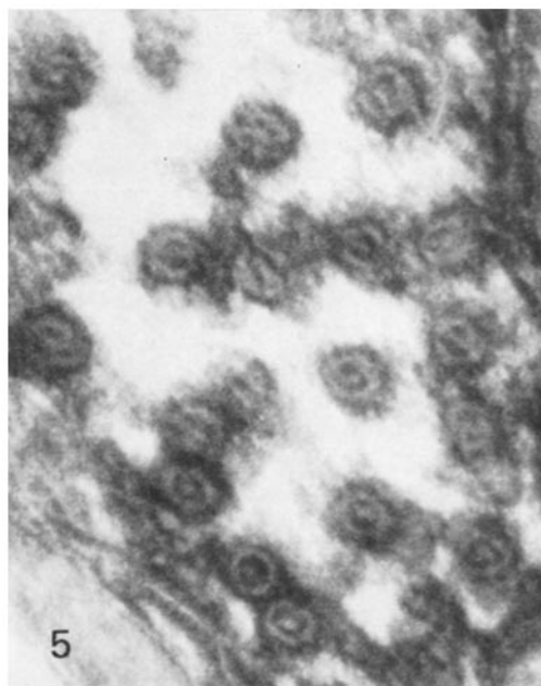
FIGURE 5 The outer and the inner concentric layers of microtubules are composed of globular subunits. The cytoplasmic matrix around the microtubules also demonstrates similar globular subunits. \times 228,000 .
