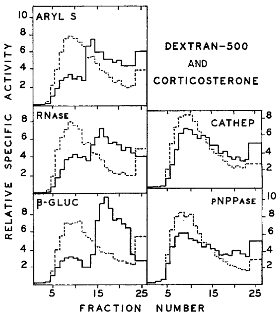
FIGURE 4 Influence of dextran-500 and corticosterone on the rate zonal sedimentation distribution pattern of muscle acid hydrolases. Animals were treated with dextran-500 (400 mg/100 g body weight) and corticosterone (15 mg) for 4 consecutive days as described in text. Experimental distribution patterns represent the average of two experiments. Dotted lines show normal distributions.
