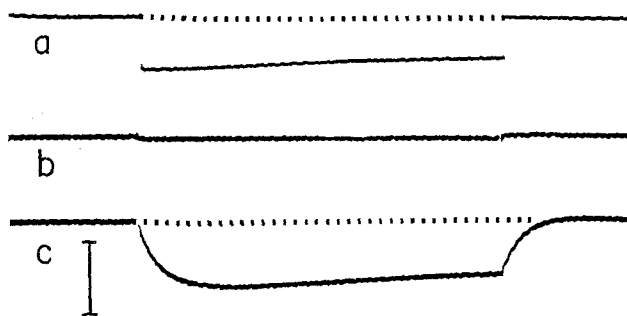
FIGURE 4 Electrical records for cells in Fig. 3. Current pulse in one lens cell ( a , 3.5 \times 10^{-8} A for 0.95 sec) produced electrotonic potential change inside ( c ), but not just outside ( b ) the second lens cell. Resting potential of second lens cell, 11 mv. Voltage calibration for b and c , 10 mv.
