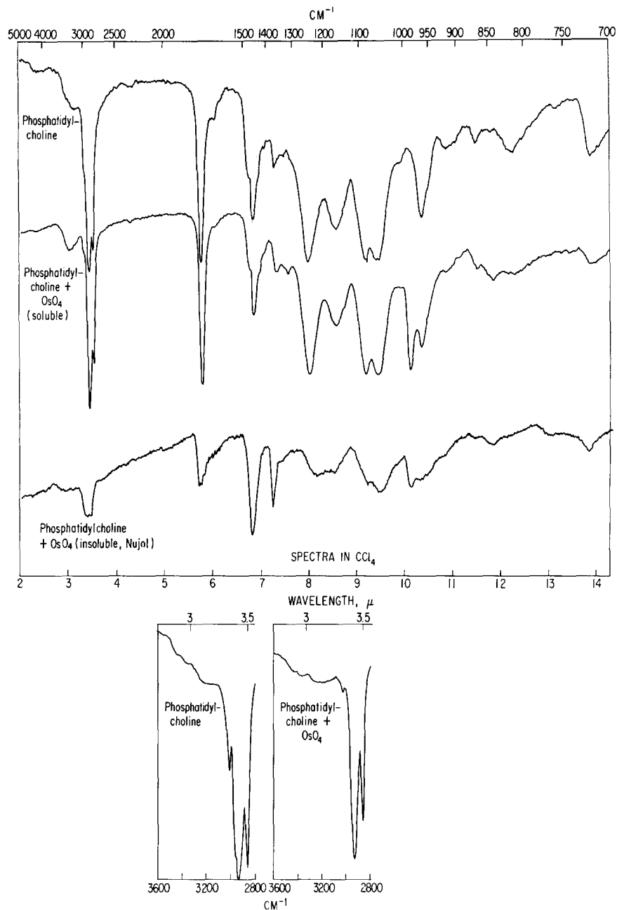
FIGURE 5 Infrared spectra of \text{CCl}_4 solutions of di-11-octadecenoyl phosphatidyleholine and its methanol-soluble osmium derivative. The spectrum of the methanol-insoluble osmium derivative was obtained as a mull in Nujol. The osmium derivatives show no increase in absorption in the hydroxyl region ( 3 \mu ) (See Table I). The phospholipids were dried in vacuo over \text{P}_2\text{O}_5 to remove water of hydration.
