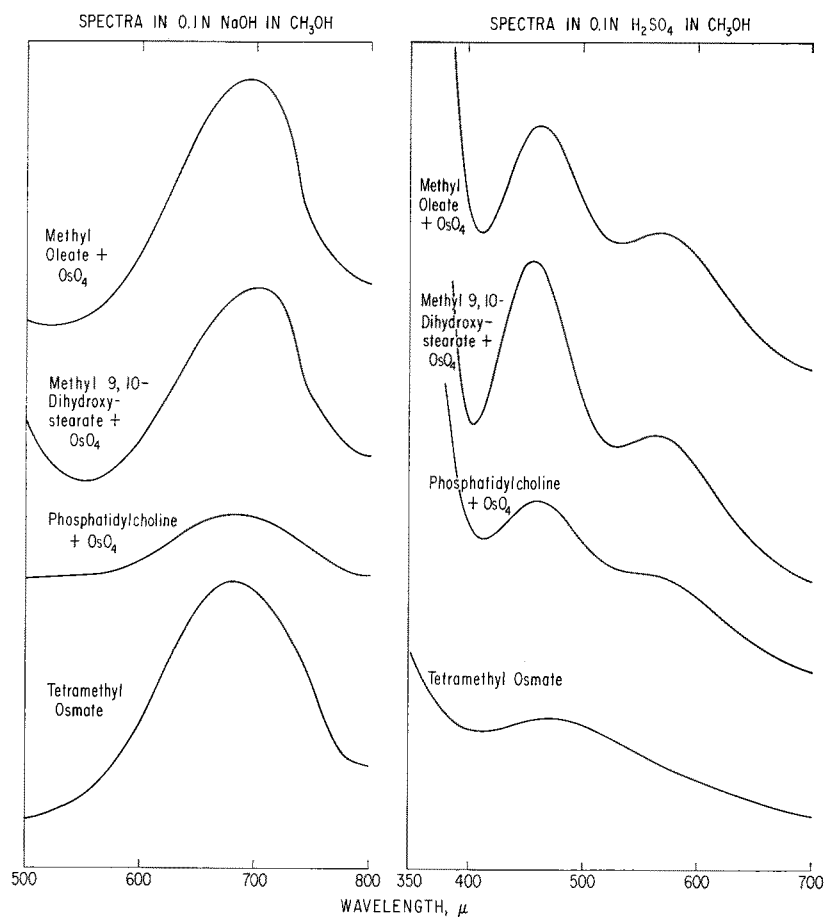
FIGURE 6 Visible spectra in acidic and alkaline methanol of tetramethyl dipotassium osmate and the osmium derivatives of methyl oleate, methyl 9,10-dihydroxystearate, and di-11-octadecenyl phosphatidylcholine.
