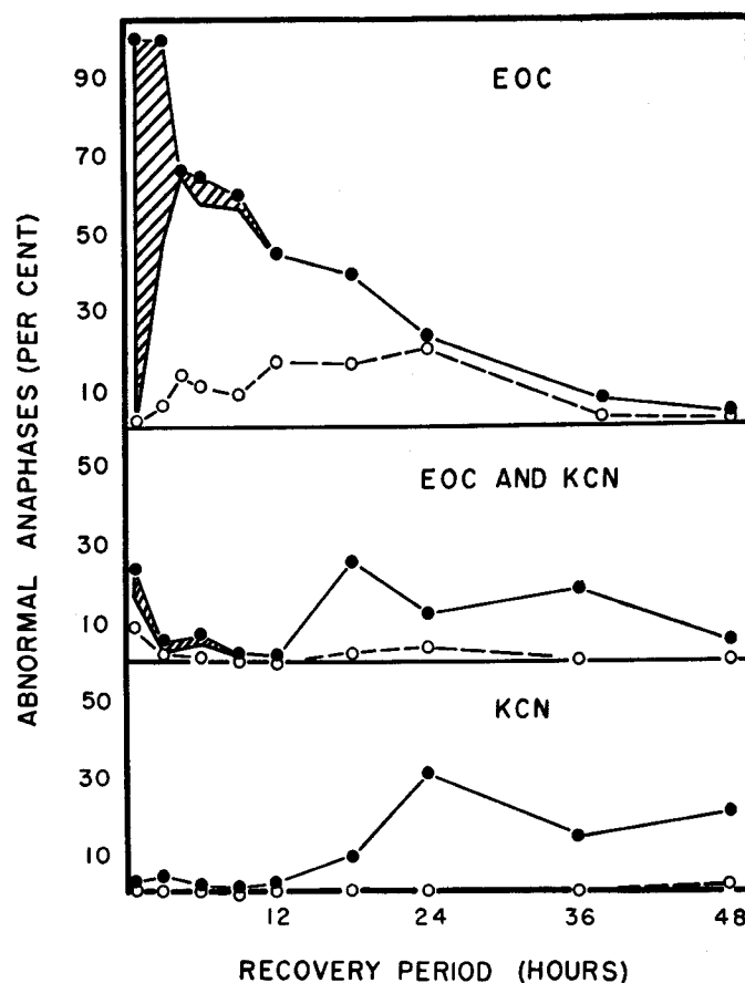
FIG. 2. The percentages of abnormal anaphases observed at different times after treatment with 8-ethoxycaffeine (EOC) and potassium cyanide (KCN) alone and in combination. ●—● = anaphases with sticky bridges and/or structural chromosome changes (total percentages of abnormal anaphases). ○---○ = anaphases with breaks localized in the nucleolar constriction. Striped area = anaphases with sticky bridges.
