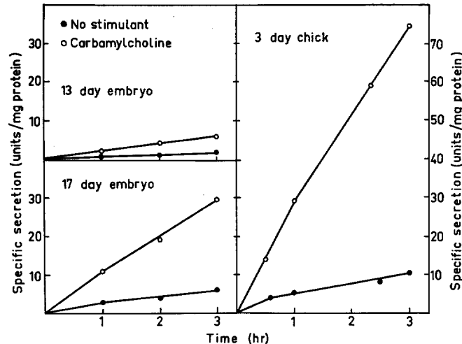
FIGURE 2 Comparison of the specific secretory rates of pancreas at various stages of development. Each vessel contained 2 pancreases in 3.0 ml of medium for the 3 day chick and in 2.0 ml for the 17 day embryo. Ten pancreases from 13-day embryos were incubated per vessel with 3.0 ml of medium from which soybean trypsin inhibitor was omitted. In the experiment on the 13-day pancreas, amylase was determined by the iodometric method but the results presented above have been converted to Bernfeld units. The carbamylcholine concentration was 10^{-4} M in all experiments.
