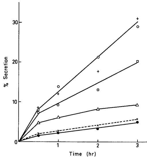
FIGURE 1 Effect of secretory stimulants on the 3 day chick pancreas. Each vessel contained 2 pancreases in 3.0 ml of medium. Stimulants were added to the medium before the introduction of the pancreases to give a final concentration of 10^{-4} M. Control, ●; Epinephrine, ×; Pilocarpine, □; Acetylcholine, △; Acetylcholine + Eserine, +; Carbamylcholine, ○.
