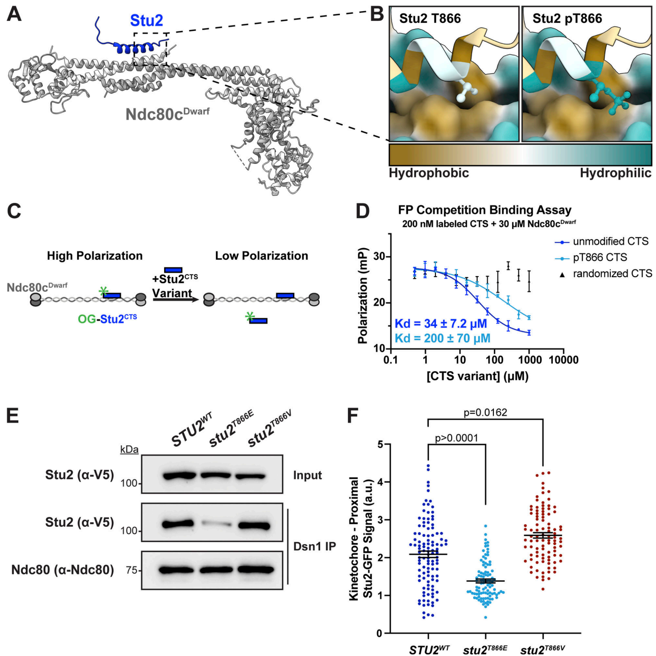
Figure 2. Phosphorylated T866 decreases binding of Stu2 to Ndc80c. (A) The crystal structure of Stu2 C-terminus bound to Ndc80c Dwarf (PDB 7KDF); see Zahm et al. (2021). Ndc80c Dwarf in grey, Stu2 C-terminus in blue. (B) Zoom in of crystal structure showing hydrophobicity of Stu2 and Ndc80c amino acids rendered using ChimeraX on the Kyte–Doolittle scale (kdHydrophobicity). Ndc80c proteins in surface representation; Stu2 in ribbon representation. Left: Unmodified Stu2 T866 as in PDB 7KDF. Right: Modeling of Stu2 pT866 . (C) Schematic representation of fluorescence polarization competition assay. Oregon Green-labeled Stu2 CTS peptide prebound to Ndc80c Dwarf was then incubated with unlabeled Stu2 peptide with or without pT866, and fluorescence polarization was measured. (D) A Stu2 CTS peptide (855–888), a Stu2 CTS peptide containing a phosphothreonine at position 866, and a peptide with a randomized CTS sequence were subjected to serial twofold dilutions, and each dilution was mixed 1:1 with a solution containing 30 \mu M Ndc80c Dwarf and 200 nM Oregon Green-labeled CTS peptide, also in resuspension buffer. Fluorescence polarization was measured in triplicate in 96-well plates. Error bars are SD. K_d calculated with four parameter logistic curve fitting in Prism. (E) Exponentially growing stu2-AID cultures expressing an ectopic copy of STU2 ( STU2 WT , M622; stu2 T866E , M1448; stu2 T866V , M4398) as well as DSN1-6His-3Flag at the genomic locus were treated with auxin 30 min prior to harvesting. Kinetochore particles were purified from lysates by anti-Flag immunoprecipitation (IP) and analyzed by immunoblotting. (F) Exponentially growing stu2-AID pMET-CDC20 cultures with an ectopically expressed STU2-GFP allele ( STU2 WT -GFP, M2599; stu2 T866E -GFP, M2600; and stu2 T866V -GFP, M4447) that also contained SPC110-mCherry (spindle pole) were shifted to auxin-containing media to degrade Stu2-AID and supplemented with methionine to arrest cells in metaphase by depleting Cdc20. Cells were fixed and imaged to determine kinetochore-proximal Stu2-GFP. Bars represent the mean of n = 96 –111 individual measurements. Error bars are SEM. P values from two-tailed unpaired t tests. Source data are available for this figure: SourceData F2.
